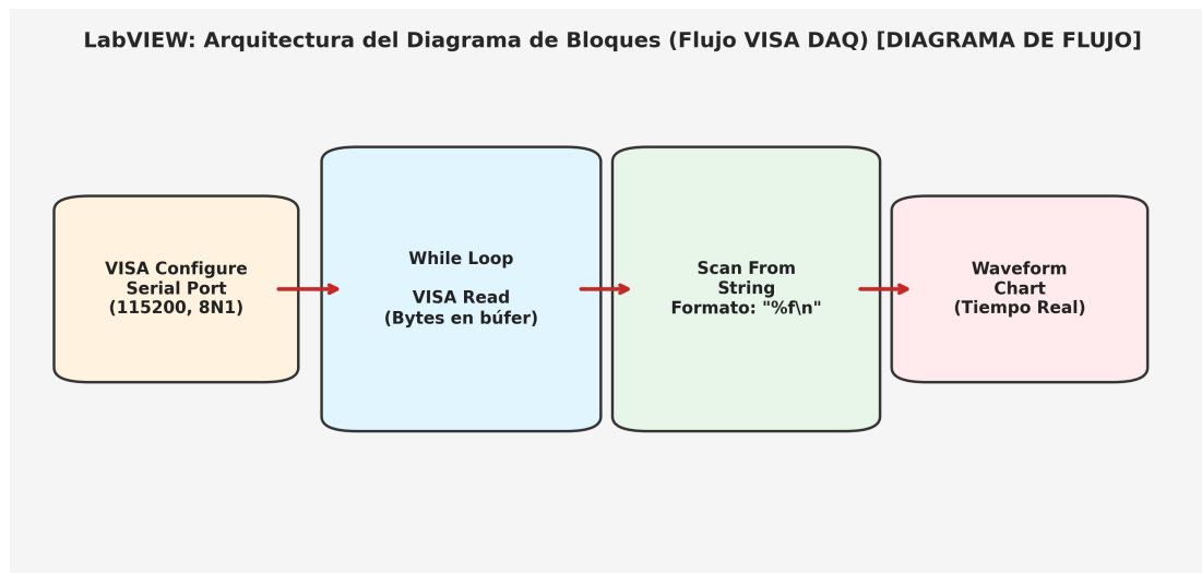
Figura 6: Diagrama de Bloques conceptual del Instrumento Virtual en LabVIEW implementando el protocolo VISA Configure, While Loop, VISA Read y Scan from String.
