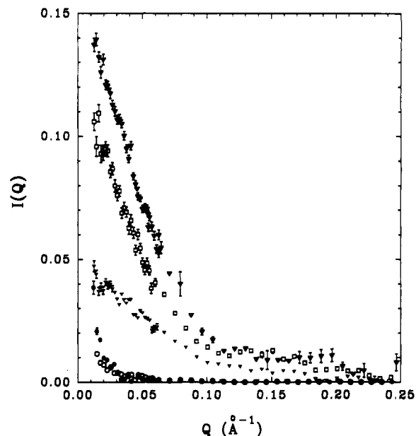
FIGURE 2: Neutron scattering data for 4\text{Ca}^{2+}\cdot\text{TnC}_{78\%d}\cdot\text{TnI} collected on beamline NG3 at NIST with (▽) 0%, (□) 20%, (●) 40%, (○) 90%, and (○) 100% \text{D}_2\text{O} . The 0%, 20%, and 40% \text{D}_2\text{O} samples contained 2 M urea, and the 90% and 100% \text{D}_2\text{O} samples contained 3 M urea. Data are on the same arbitrary normalization scale, but not corrected for concentration or path-length differences.
