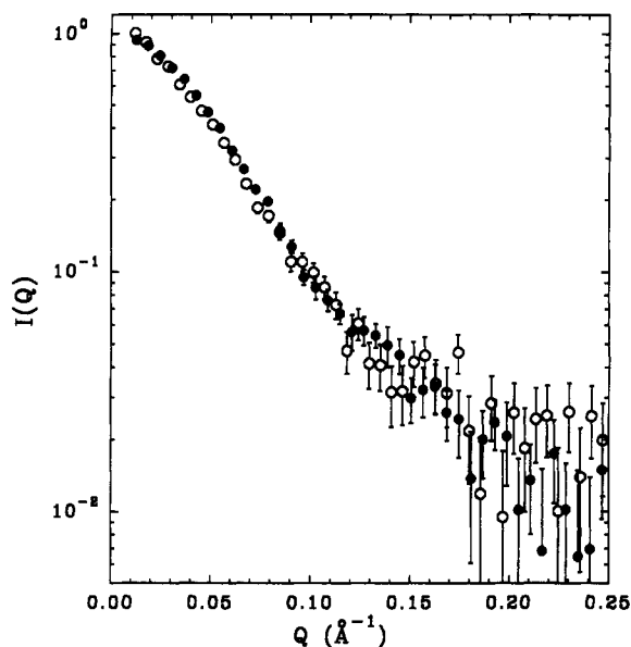
FIGURE 1: Comparison of X-ray scattering data from the 4\text{Ca}^{2+}\cdot\text{TnC}_{78\%d}\cdot\text{TnI} complex, \approx 3 mg/mL protein, in buffer A (O) with \text{H}_2\text{O} and 0 M urea and (●) in buffer A with \text{D}_2\text{O} and 3 M urea.
