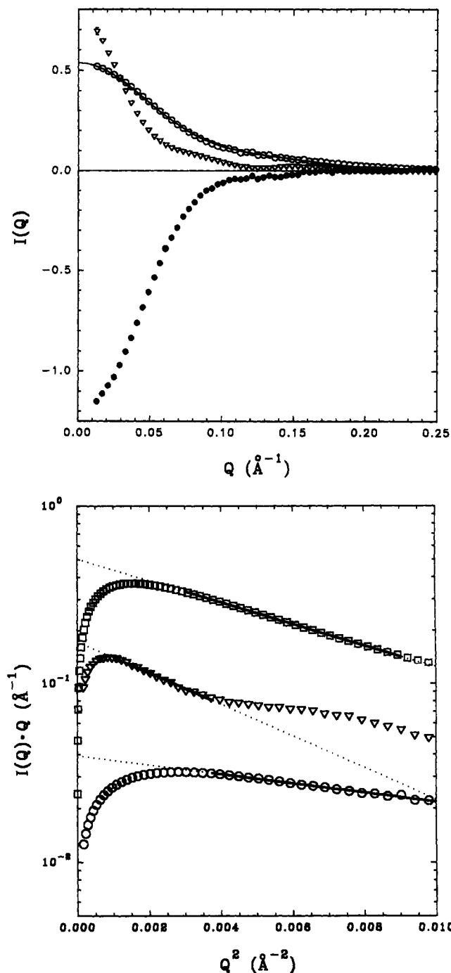
FIGURE 3: (Top) Basic scattering functions calculated using eq 2 for 4\text{Ca}^{2+}\cdot\text{TnC}_{78\%} (O), TnI ( \nabla ), and the cross-term ( \bullet ) between the two proteins in the complex. The solid line is the calculated scattering curve from the known crystal structure of 2\text{Ca}^{2+}\cdot\text{TnC} (Herzberg & James, 1985). (Bottom) Guinier showed that for a "rod-shaped" particle, a plot of \ln I(Q)\cdot Q vs Q^2 is linear at certain small Q values, with a slope proportional to the mean R_c value of the scattering particle. Shown here are the Guinier plots for 4\text{Ca}^{2+}\cdot\text{TnC} (O) and TnI ( \nabla ) (using the basic scattering functions) and for 4\text{Ca}^{2+}\cdot\text{TnC}\cdot\text{TnI} ( \square ) (using the X-ray scattering data). The solid lines show the regions of the Guinier plots fitted for each profile, and the dotted lines are extrapolations of those fits. The roll-over observed at the lowest Q values is expected because of the finite lengths of the rod-shaped particles. The linearity is also expected to break down at high Q values, and the Q value at which this breakdown occurs is indirectly proportional to the R_c value (as we observe for these data sets).
