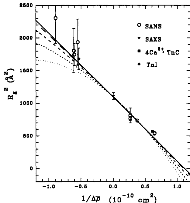
FIGURE 5: Stuhrmann plot ( R_g^2 versus 1/\Delta\bar{\rho} ). The line fits were determined from eqs 4 and 5 by assuming fixed R_g values of 23.9 and 41 Å for 4\text{Ca}^{2+}\cdot\text{TnC} and TnI, respectively, and varying the separation, D , of the two components. Separations are (—) 0, (---) 5, (- - -) 10, (- - -) 15, and (····) 20 Å.
