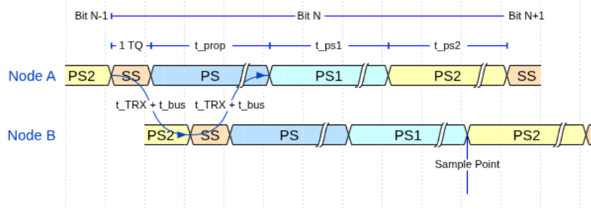
Figure 5: CAN bit time segments (SS, PS, PS1, PS2) and Sample Point (SP). The two-node layout illustrates the round-trip propagation delay ( t_{\text{TRX}} + t_{\text{bus}} each way) that PS must cover for correct arbitration.
