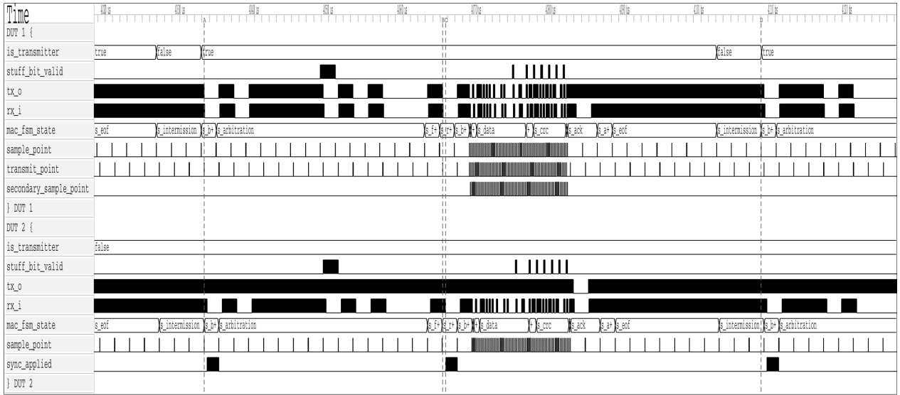
Figure 17: REQ-009. Two-node simulation of a complete FD frame. DUT 1 is the transmitter (is_transmitter = true), DUT 2 the receiver. mac_fsm_state traces show the full frame-field sequence from s_arbitration through s_eof; secondary_sample_point pulses on DUT 1 confirm TDC is active during the data phase; sync_applied pulses on DUT 2 show receiver soft-synchronisation events. After EOF both nodes traverse s_intermission and the sample-point counter accumulates 11 consecutive recessive bits, producing the idle condition and completing bus re-integration (REQ-009).
