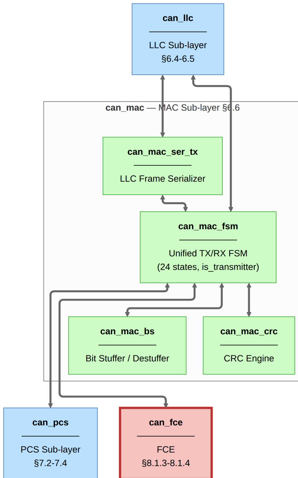
Figure 8: Implementation module decomposition. can_llc provides the Avalon-ST host interface and manages retransmission and acceptance filtering. Inside can_mac , the unified can_mac_fsm handles both TX and RX roles via a single is_transmitter flag, sharing one can_mac_bs bit stuffer and one can_mac_crc engine. can_pcs generates sample-point and SSP strobes. can_fce maintains TEC/REC counters and governs node-state transitions.
