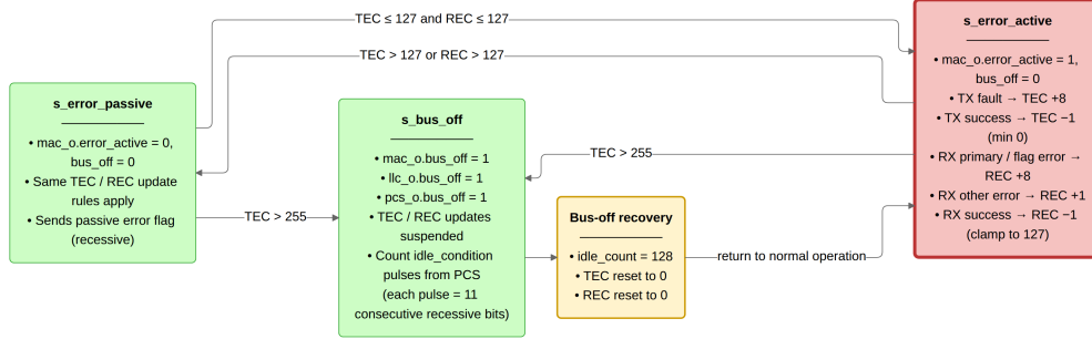
Figure 15: can_fce FSM (ISO 11898-1 sec. 8.1.4.4, Figure 43). s_error_active is the initial state after reset_i or llc_i.normal_mode . When TEC exceeds 127 or REC exceeds 127 the FCE moves to s_error_passive , clearing mac_o.error_active . If TEC exceeds 255 from either active or passive state, the FCE enters s_bus_off , asserting bus_off to the MAC, LLC, and PCS. Recovery counts 128 idle_condition pulses from the PCS (each pulse represents 11 consecutive recessive bits); on the 128th pulse TEC and REC are reset to zero and the FSM returns to s_error_active .
