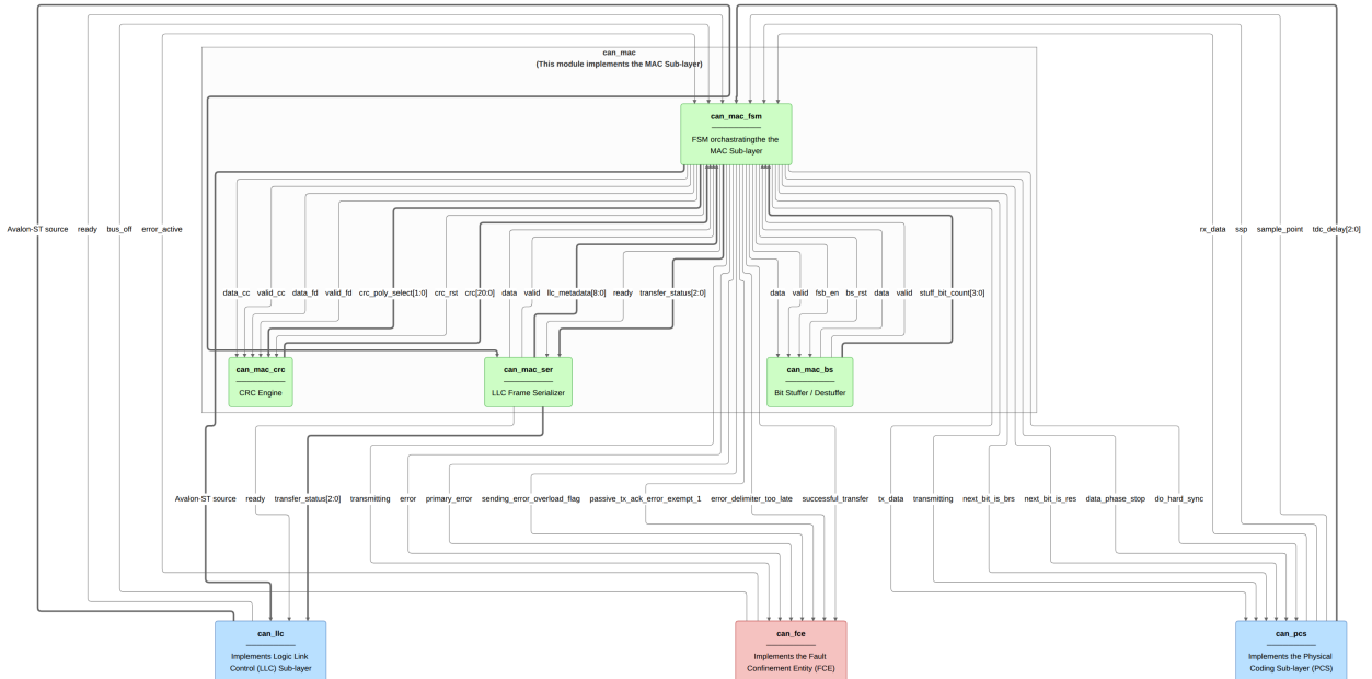
Figure 10: ‘ can_mac ’ architecture. Individual signals are shown on each directed edge. MAC-internal connections: ‘ can_mac_ser ’ feeds the serial bit stream and ‘ llc_metadata ’ to ‘ can_mac_fsm ’; ‘ can_mac_bs ’ accepts ‘ data/valid/fsb_en ’ and returns stuffed ‘ data/valid ’ plus the Gray-coded ‘ stuff_bit_count ’ for the SBC field; ‘ can_mac_crc ’ receives the dual CC/FD bit feeds and returns the running ‘ crc[20:0] ’ digest. External connections: ‘ can_llc ’ connects to the MAC on both TX (‘ tx_llc_i/o ’ via the serializer) and RX (‘ rx_llc_i/o ’ via the FSM); bit-level timing to ‘ can_pcs ’ (‘ tx_data ’, ‘ rx_data ’, sample-point strobes); fault-confinement events to/from ‘ can_fce ’ (‘ error_active ’, ‘ bus_off ’).
