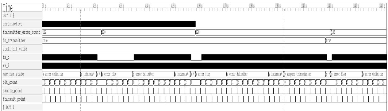
Figure 18: REQ-010/011. Error escalation waveform for DUT 1. transmitter_error_count (TEC) increments on successive error frames (13 → 128 → 136); when TEC exceeds 127, error_active deasserts and the node becomes error-passive. The mac_fsm_state trace shows s_suspend_transmission inserted after s_intermission once the node is error-passive, enforcing the mandatory 8-bit suspension period before the next transmission attempt (ISO 11898-1 §8.1.4.4).
