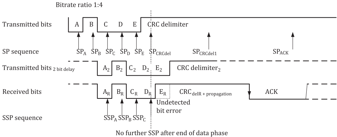
Figure 35 — End of transmitter delay compensation phase
