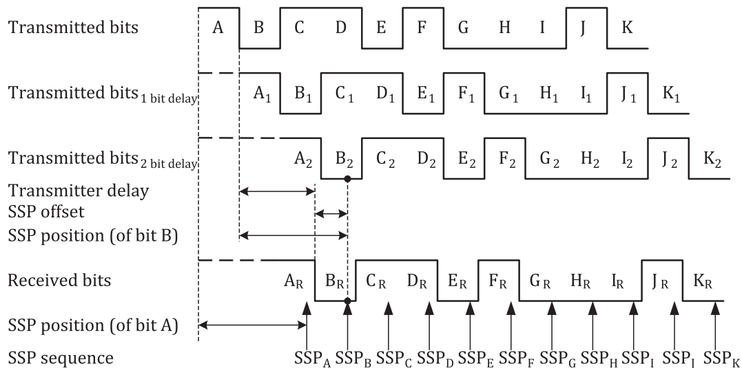
Figure 34 — Position of the secondary sample point
