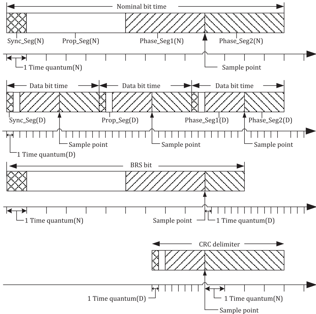
Figure 32 — Segments of nominal bit time and of data bit time
