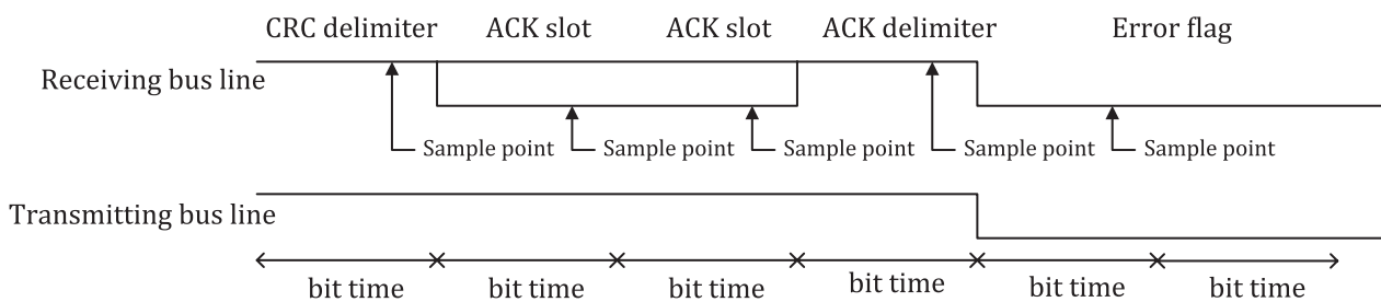
Figure 29 — CRC error in FD frames
