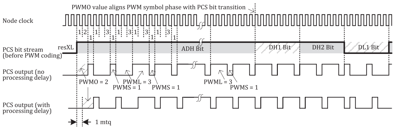
Figure 41 — Example for PWM configuration for transmitters for multiple PWM symbols per data bit
