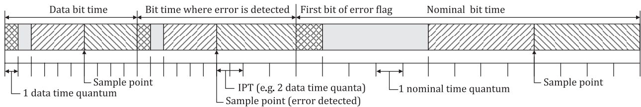
Figure 31 — Receiver detects error in data phase of an FD frame
