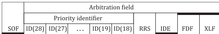
Figure 24 — SOF and arbitration field of XLFF data frame
