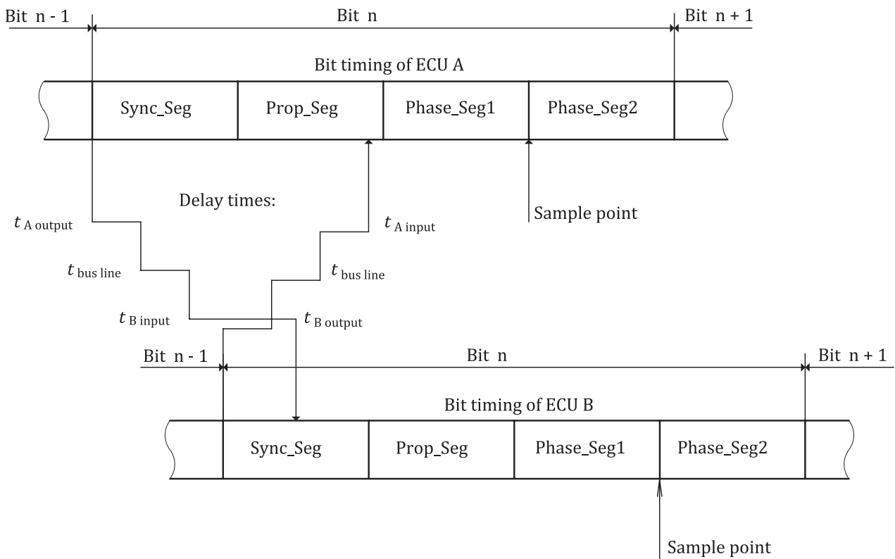
Figure 33 — Time relationship between delay times and bit time phases of CAN nodes A and B during arbitration phase
