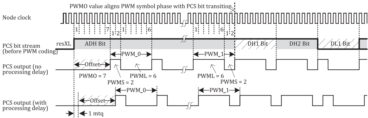
Figure 39 — Example for PWM configuration for transmitters
