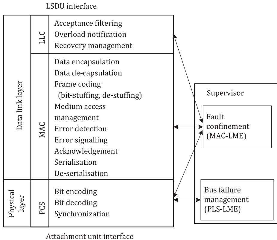
Figure 3 — Layered architecture of CAN
