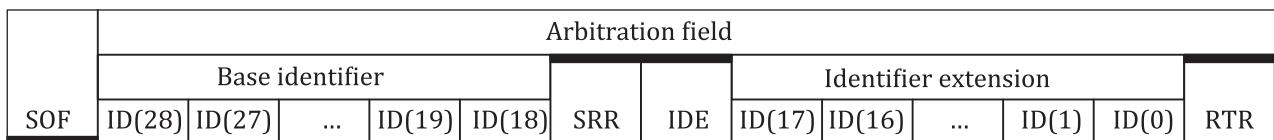
Figure 13 — SOF and arbitration field of CEFF remote frame
