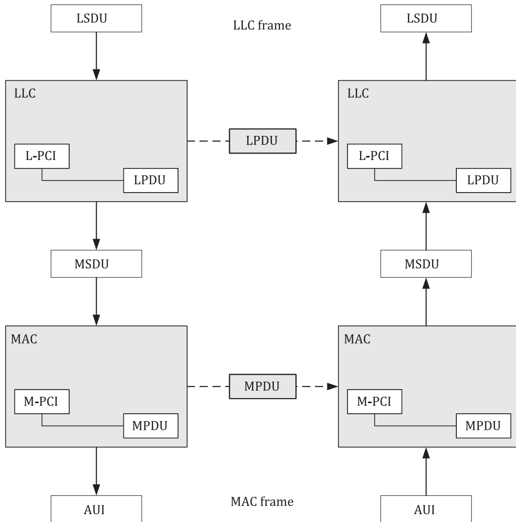
Figure 4 — Protocol layer interactions
