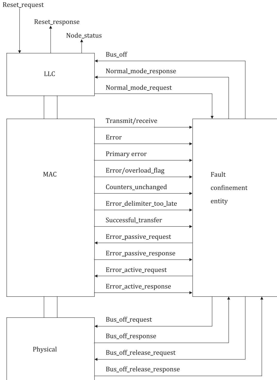
Figure 42 — Fault confinement entity interface to the OSI sub-layer entities
