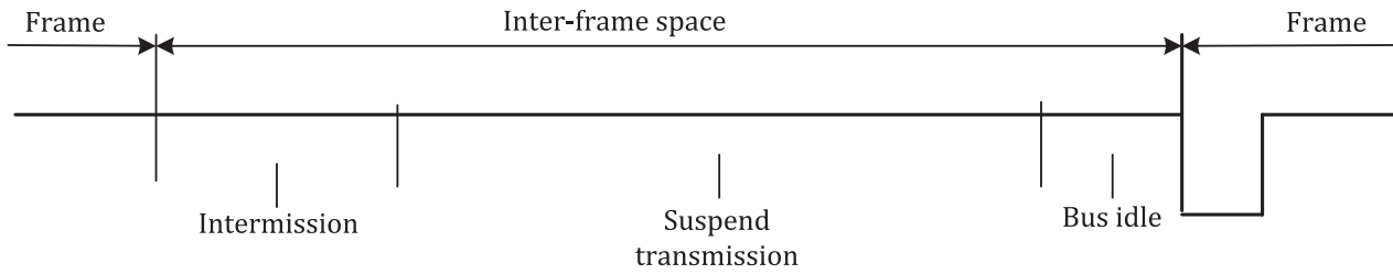
Figure 7 — Inter-frame space for error-passive nodes, which are transmitters of previous DF or RF
