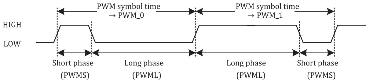
Figure 37 — PWM symbol coding definitions, example for the transmitter
