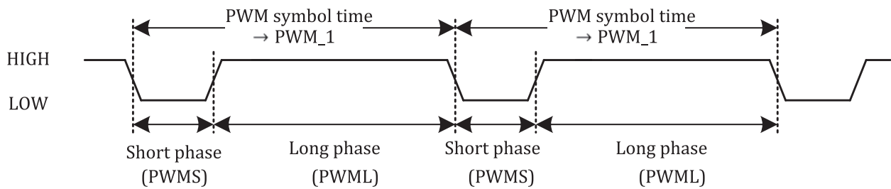
Figure 38 — PWM symbol coding definitions, example for the receiver
