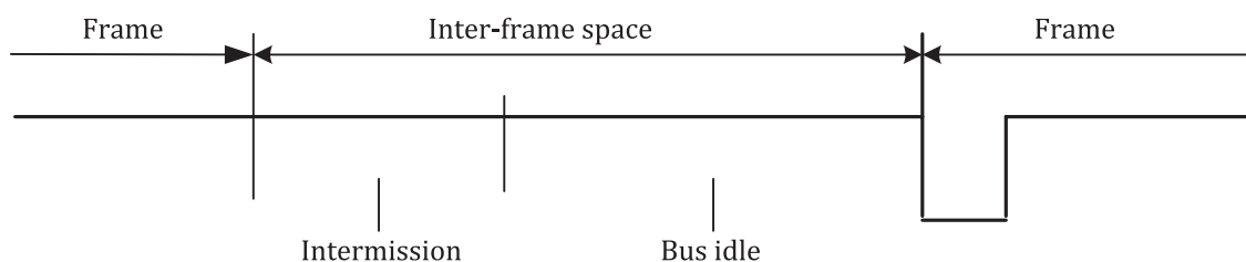
Figure 6 — Inter-frame space for nodes, which are not error-passive or are receivers of previous DF or RF
