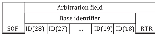
Figure 10 — SOF and arbitration field of CBFF data frame
