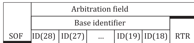
Figure 11 — SOF and arbitration field of CBFF remote frame
