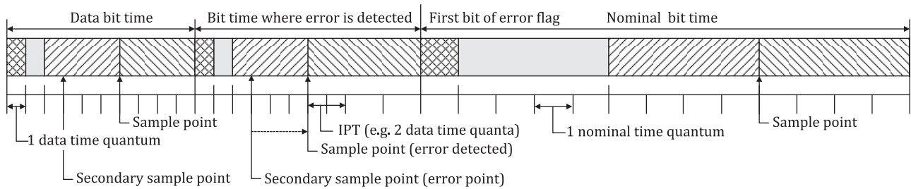
Figure 30 — Transmitter detects bit error at SSP in data phase of an FD frame
