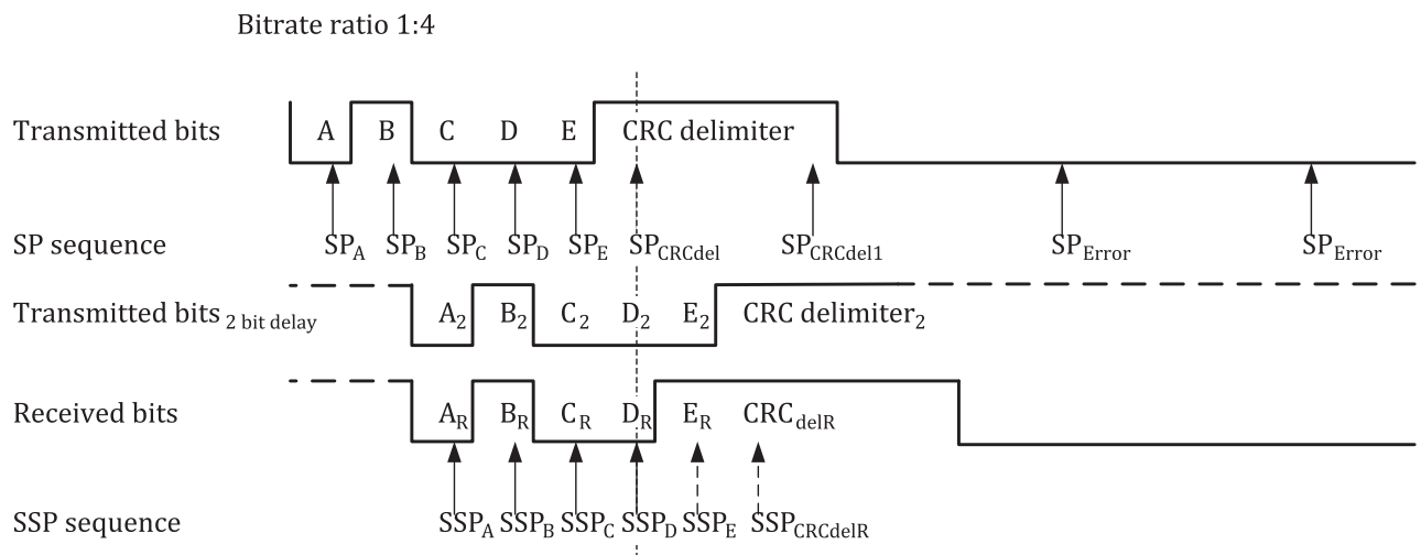
Figure 36 — Optional continuation of SSP sequence
