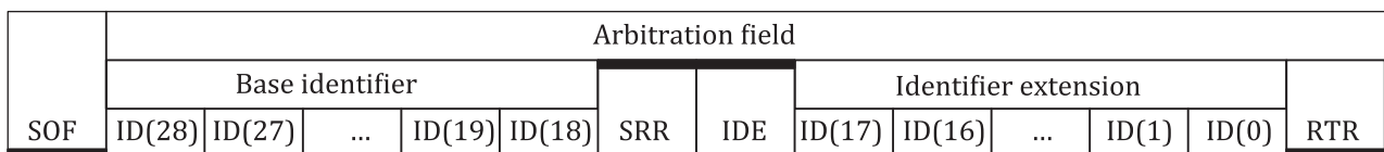
Figure 12 — SOF and arbitration field of CEFF data frame
