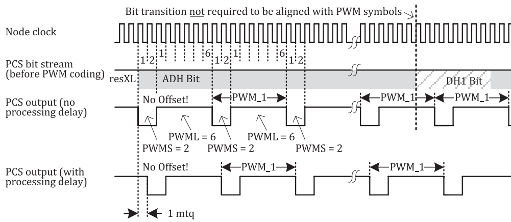
Figure 40 — Example for PWM configuration for receivers
