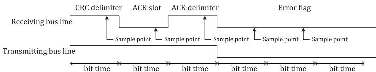
Figure 28 — CRC error in CC frames
