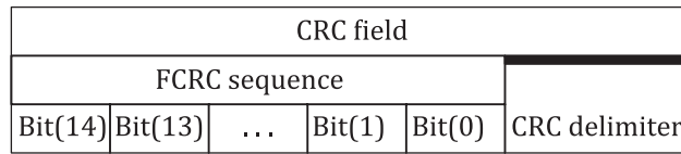
Figure 16 — CRC field in CC frame
