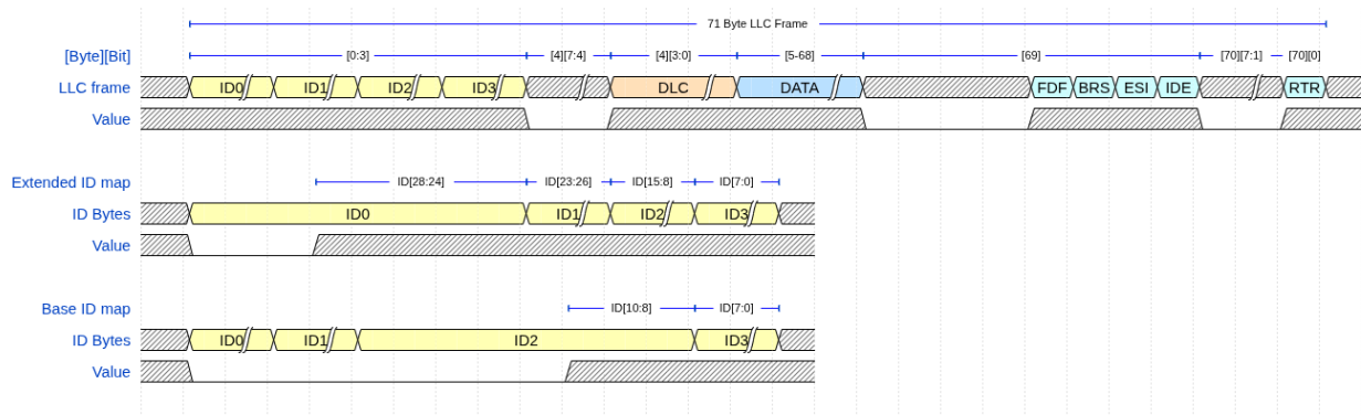
Figure 5: LLC frame format (71 bytes) at the host-MAC interface. Bytes 0-3 encode the identifier; byte 4 carries the frame-type selector FMT in bits [7:4] and DLC in bits [3:0]; bytes 5-68 carry up to 64 data bytes; byte 69 carries the FDF, BRS, ESI, and IDE control flags; byte 70 carries RTR in bit 0. The lower rows show the identifier byte mapping: for extended identifiers ID[28:24] are packed into ID0, ID[23:16] into ID1, ID[15:8] into ID2, and ID[7:0] into ID3; for base identifiers ID0 and ID1 are all zeros, ID[10:8] occupies the lower three bits of ID2, and ID[7:0] fills ID3.
