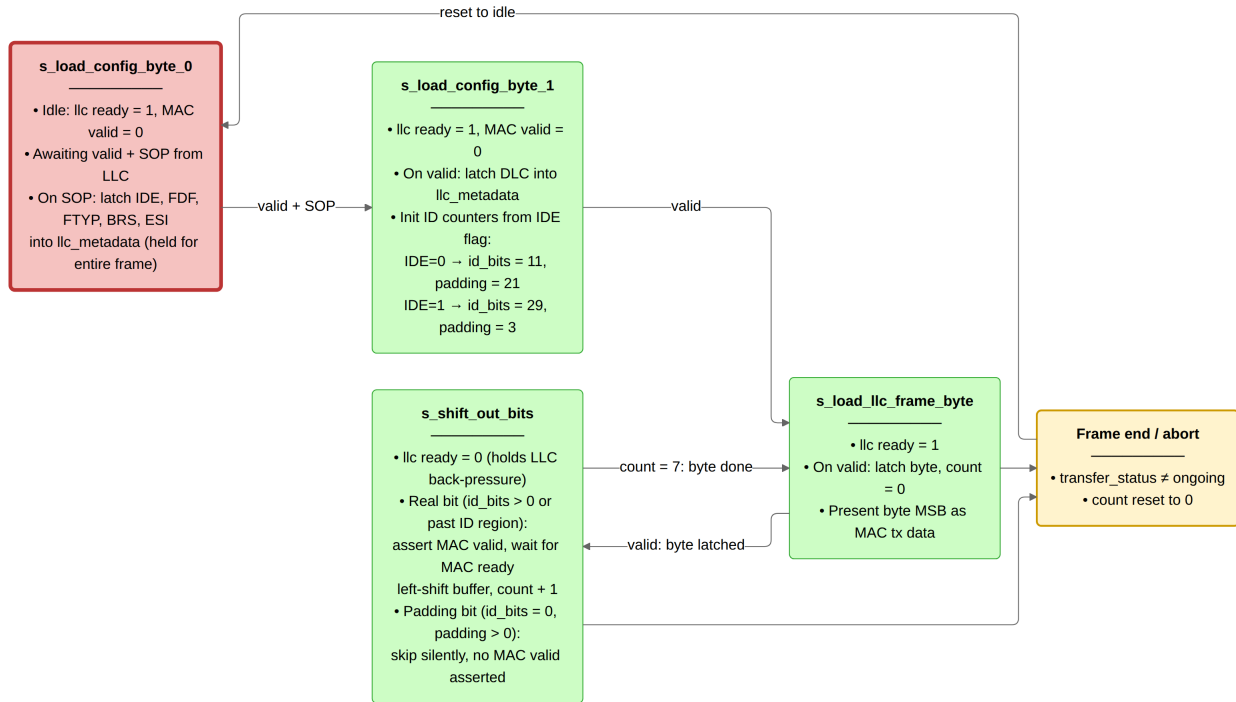
Figure 15: can_mac_ser (4 states). Config bytes carry frame metadata (IDE, FDF, FTYP, BRS, ESI, DLC); these are latched once and held stable for the entire frame. In s_shift_out_bits real ID and data bits are driven one per MAC FSM ready pulse, while unused padding bits in the 32-bit ID field are skipped silently. Any transfer_status ≠ ongoing signal from the MAC FSM returns the serializer to s_load_config_byte_0 from any state.
