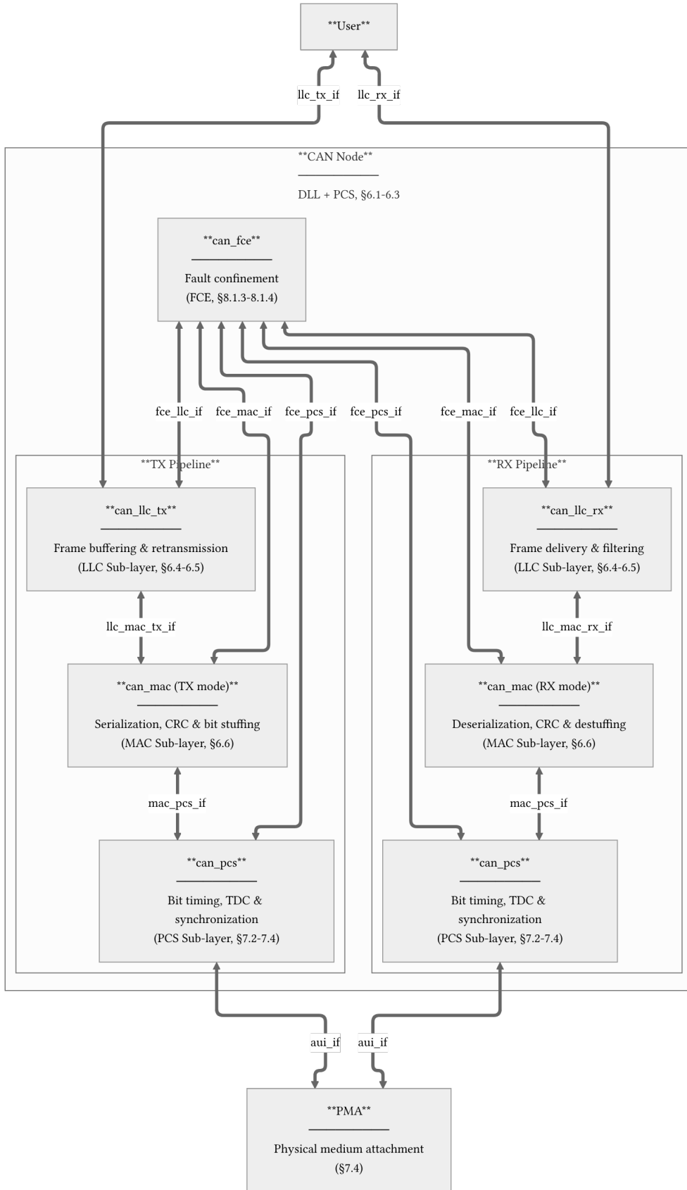
Figure 9: CAN node decomposition across LLC, MAC, PCS, FCE, and PMA boundaries. Interface definitions are provided for llc_tx_if (Table ??), llc_rx_if (Table ??), llc_mac_tx_if (Table ??), llc_mac_rx_if (Table ??), mac_pcs_if (Table ??), auif (Table ??), fce_llc_if (Table ??), fce_mac_if (Table ??), and fce_pcs_if (Table ??).
