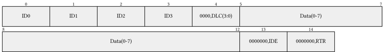
Figure 10: Current LLC frame format (15 bytes). ID byte encoding is defined in Table 4.
