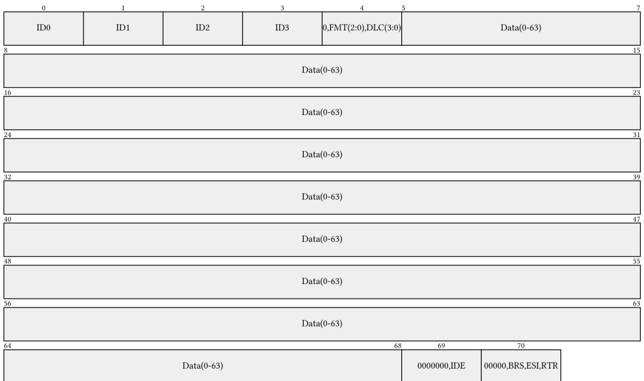
Figure 11: Revised LLC frame format with FD support, shown at maximum length (71 bytes). The FMT field selects frame type; BRS and ESI repurpose reserved bits in the final byte. ID byte encoding is defined in Table 4.
