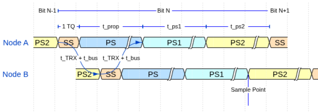
Figure 6: CAN bit time structure. One bit consists of SYNC_SEG (SS) which is 1 Time Quantum (TQ) long, PROP_SEG (PS), PHASE_SEG1 (PS1), and PHASE_SEG2 (PS2). The sample point (SP) sits at the PHASE_SEG1/PHASE_SEG2 boundary. The figure illustrates a to-node synchronised bus with bus wire delay t_{bus} and transceiver delay t_{TRX} .
