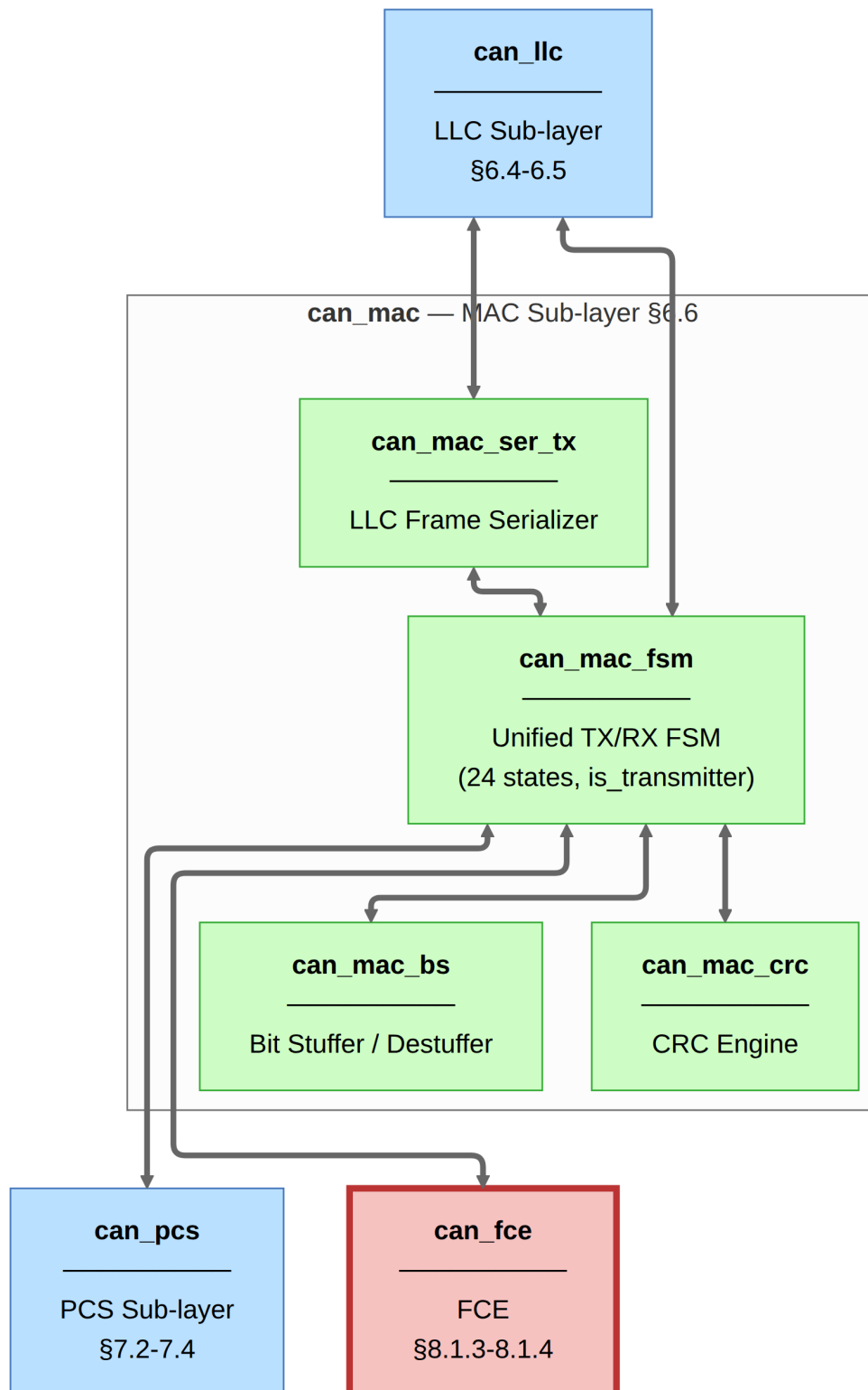
Figure 12: can_mac module topology. Each bidirectional edge represents one or more interface signals between the connected modules. The detailed per-signal breakdown is given in Figure ??.
