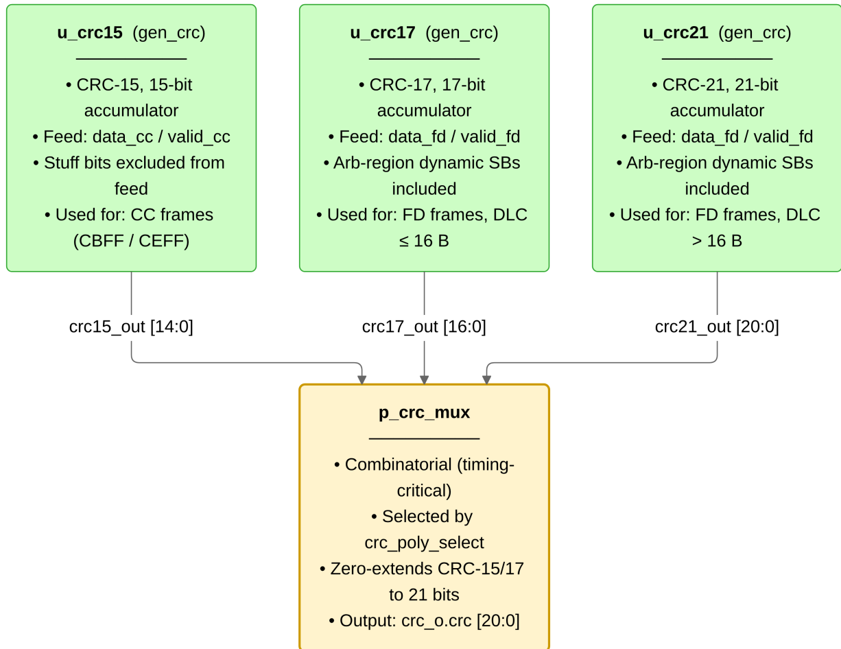
Figure 17: can_mac_crc dataflow. Three gen_crc instances accumulate in parallel on every clock: u_crc15 is fed by data_cc/valid_cc (CC bit stream, stuff bits excluded); u_crc17 and u_crc21 are both fed by data_fd/valid_fd (FD bit stream, dynamic stuff bits included in the arbitration region). The combinatorial mux p_crc_mux selects the active engine result based on crc_poly_select and zero-extends it to the common 21-bit output. reset_i reinitializes all three engines simultaneously.
