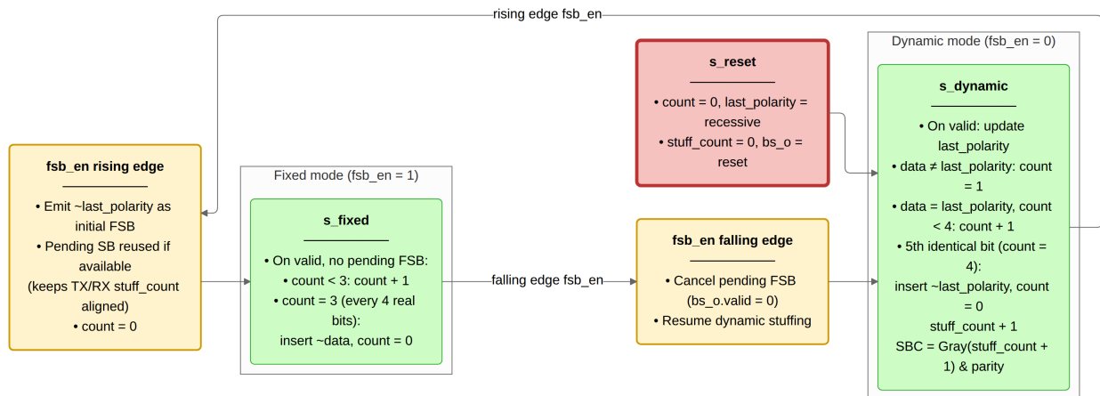
Figure 16: can_mac_bs (2 modes). Dynamic mode counts consecutive identical bits and emits an inverse stuff bit on the 5th (count = 4), updating the Gray-coded SBC. Fixed mode is entered on the rising edge of fsb_en , which immediately emits the initial FSB; thereafter one FSB is emitted every 4 real bits (count = 3). The falling edge of fsb_en cancels any pending FSB and returns to dynamic mode. stuff_count and the SBC output are maintained continuously across both modes.
