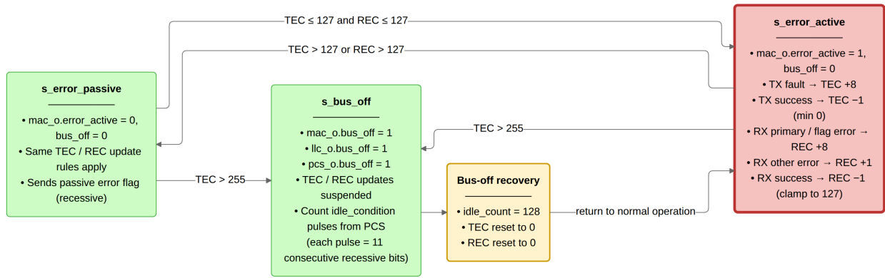
Figure 18: can_fce FSM (ISO 11898-1 sec. 8.1.4.4, Figure 43). s_error_active is the initial state after reset_i or llc_i.normal_mode. When TEC exceeds 127 or REC exceeds 127 the FCE moves to s_error_passive, clearing mac_o.error_active. If TEC exceeds 255 from either active or passive state, the FCE enters s_bus_off, asserting bus_off to the MAC, LLC, and PCS. Recovery counts 128 idle_condition pulses from the PCS (each pulse represents 11 consecutive recessive bits); on the 128th pulse TEC and REC are reset to zero and the FSM returns to s_error_active.
