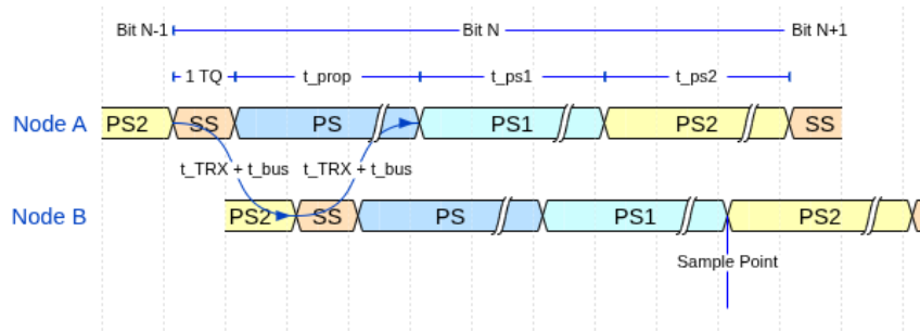
Figure 5: CAN bit time segments (SS, PS, PS1, PS2) and Sample Point (SP). The two-node layout illustrates the round-trip propagation delay ( t_{TRX} + t_{bus} each way) that PS must cover for correct arbitration.
