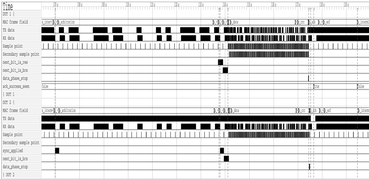
Figure 19: Two-node simulation of a complete FD frame transmission in can_mac_pcs_fce_tb. DUT 2 hard-synchronizes on SOF at A. DUT 1 measures the TDC loopback delay between B and C. Both nodes switch to data-phase bit timing at the BRS sample point at D. DUT 1 switches back to nominal bit timing at the CRC delimiter sample point at E. DUT 2 drives the ACK slot dominant at F, DUT 1 samples the dominant ACK at G and latches ack_success_seen. Transmission ends at H.
