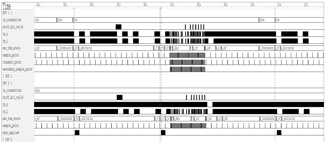
Figure 17: REQ-009. Two-node simulation of a complete FD frame. DUT 1 is the transmitter ( is_transmitter = true ), DUT 2 the receiver. mac_fsm_state traces show the full frame-field sequence from s_arbitration through s_eof ; secondary_sample_point pulses on DUT 1 confirm TDC is active during the data phase; sync_applied pulses on DUT 2 show receiver soft-synchronisation events. After EOF both nodes traverse s_intermission and the sample-point counter accumulates 11 consecutive recessive bits, producing the idle condition and completing bus re-integration (REQ-009).
