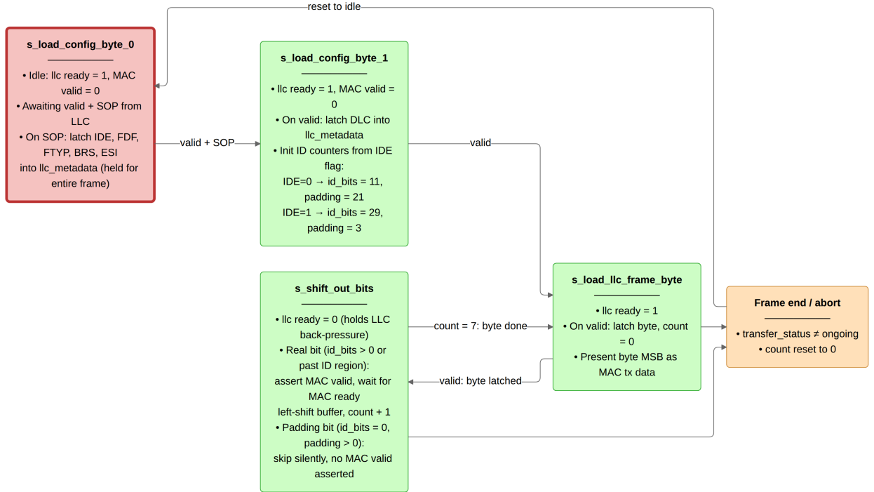
Figure 14: can_mac_ser FSM (four states) serializing the internal LLC frame to the MAC bit stream. Unused padding bits in the 32-bit ID field are skipped silently.
