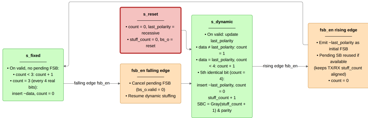
Figure 15: can_mac_bs operating in dynamic and fixed stuffing modes. A pending dynamic stuff bit at the rising edge of fbs_en is promoted to the initial FSB rather than suppressed.
