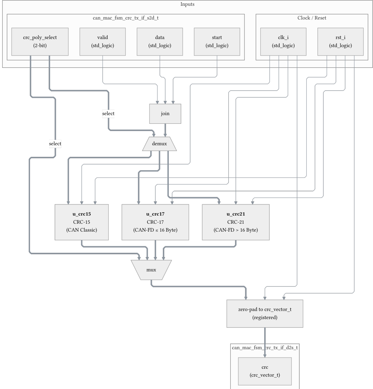
Figure 9: can_mac_crc_tx selection architecture. Three CRC engine instances run in parallel. The FSM drives crc_poly_select to gate valid and start per engine so that only the selected polynomial accumulates data. A registered output mux selects the active engine result and zero-pads it into the common crc_vector_t format.
