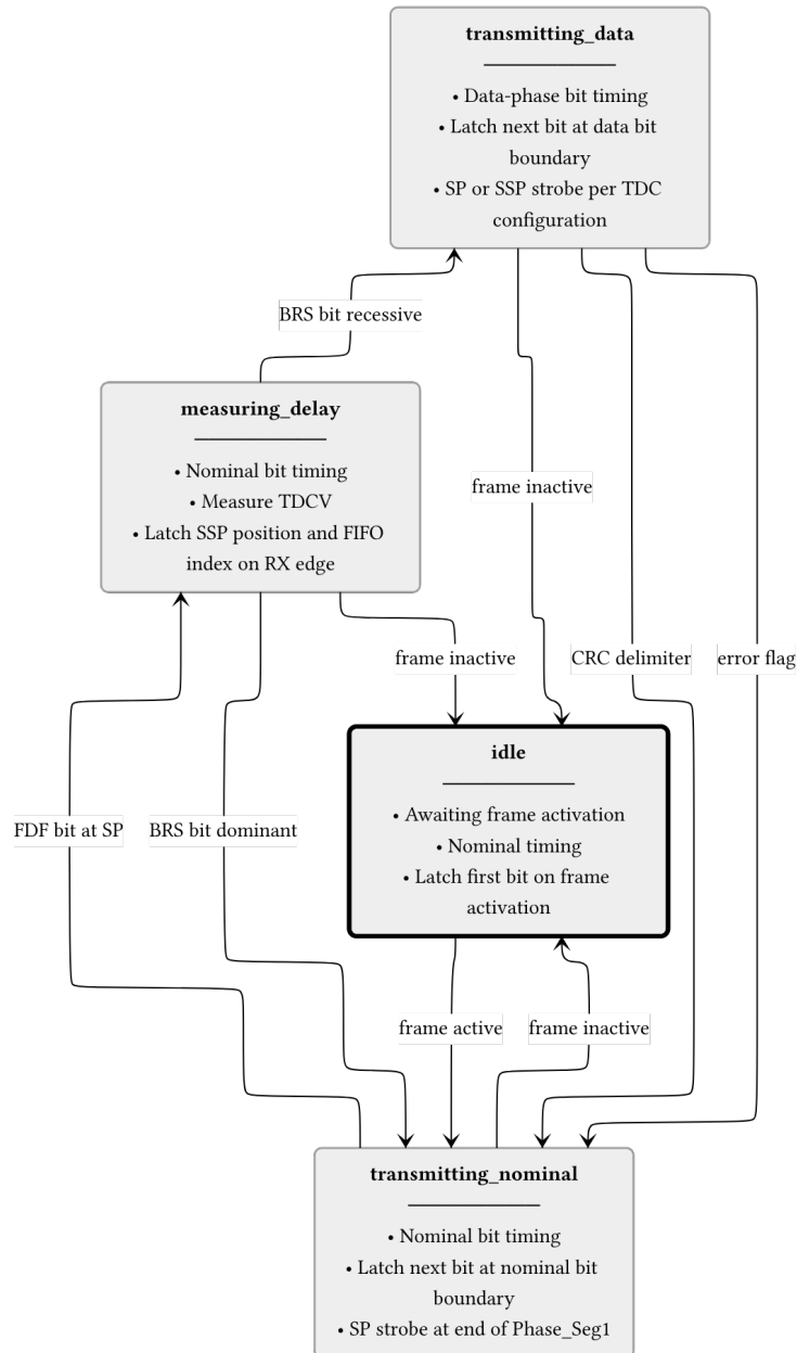
Figure 11: can_pcs_tx FSM. The measuring_delay state is entered on the FDF sample point to measure TDCV (Transmitter Delay Compensation Value, [1], sec. 7.3.4)]. The BRS bit boundary determines whether data-phase timing is used. All non-idle states return to idle when the frame becomes inactive.
