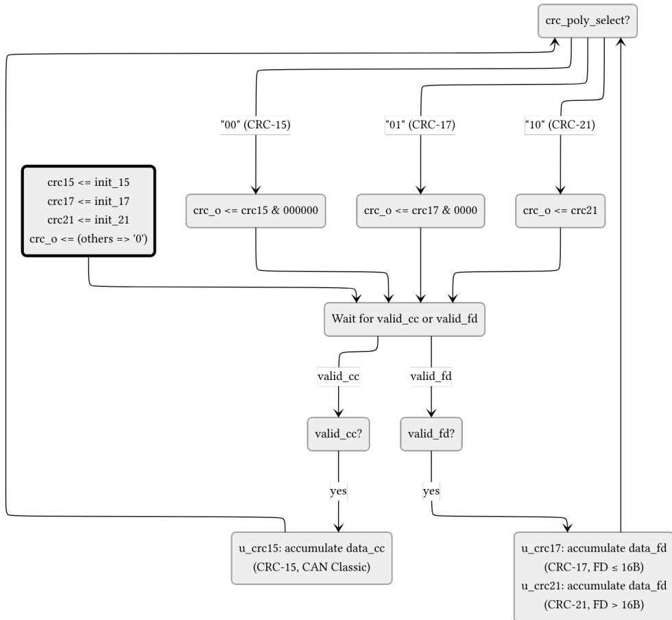
Figure 8: can_mac_crc data path diagram. Three parallel gen_crc instances accumulate continuously: data_cc drives CRC-15 via valid_cc, while data_fd drives both CRC-17 and CRC-21 via valid_fd. The output register selects the active engine result based on crc_poly_select and left-aligns it to 21 bits. The external rst signal reinitializes all three engines and the output register.
