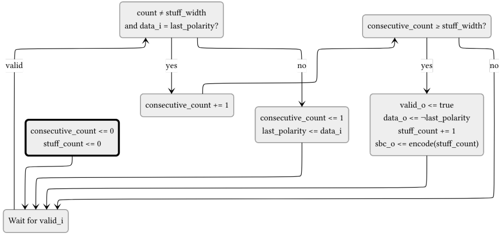
Figure 7: can_mac_bs data path diagram. When valid and data = last_polarity , consecutive_count increments. Otherwise it restarts at 1 with last_polarity updated to data . When consecutive_count reaches stuff_width (5 in dynamic mode, 4 in fixed mode), valid and inverted data are driven and stuff_count increments. The to_gray() + calc_parity() block encodes stuff_count into the stuff_bit_count output. The external rst signal resets consecutive_count and stuff_count to zero. The fixed_bit_stuffing_en signal selects between dynamic and fixed modes. All outputs are registered.
