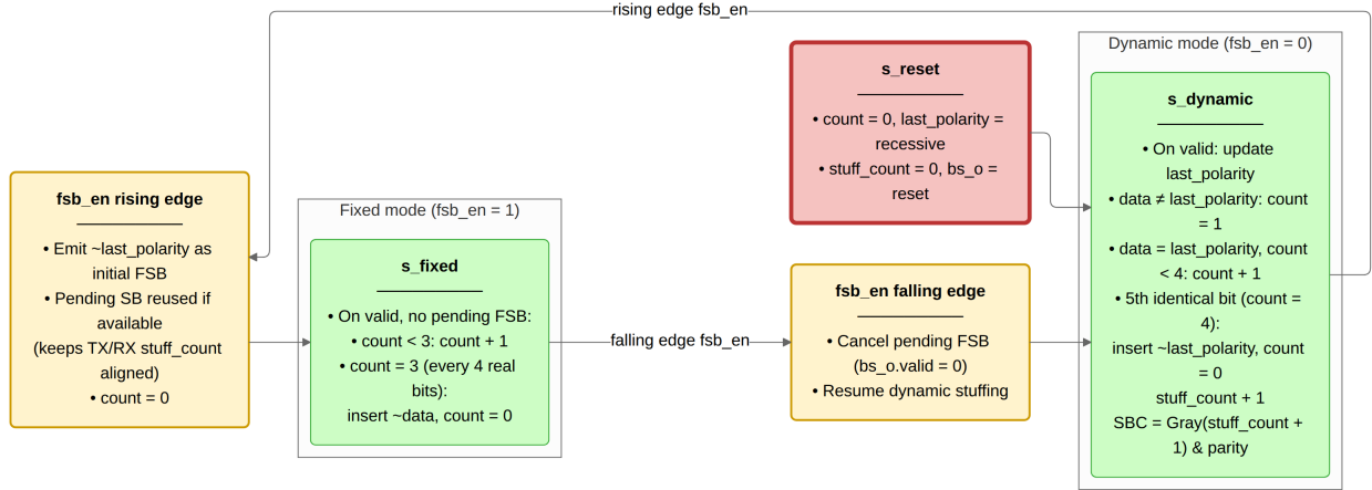
Figure 14: can_mac_bs (2 modes). Dynamic mode counts consecutive identical bits and emits an inverse stuff bit on the 5th ( count = 4 ), updating the Gray-coded SBC. Fixed mode is entered on the rising edge of fsb_en , which immediately emits the initial FSB. Thereafter one FSB is emitted every 4 real bits ( count = 3 ). The falling edge of fsb_en cancels any pending FSB and returns to dynamic mode. stuff_count and the SBC output are maintained continuously across both modes.
