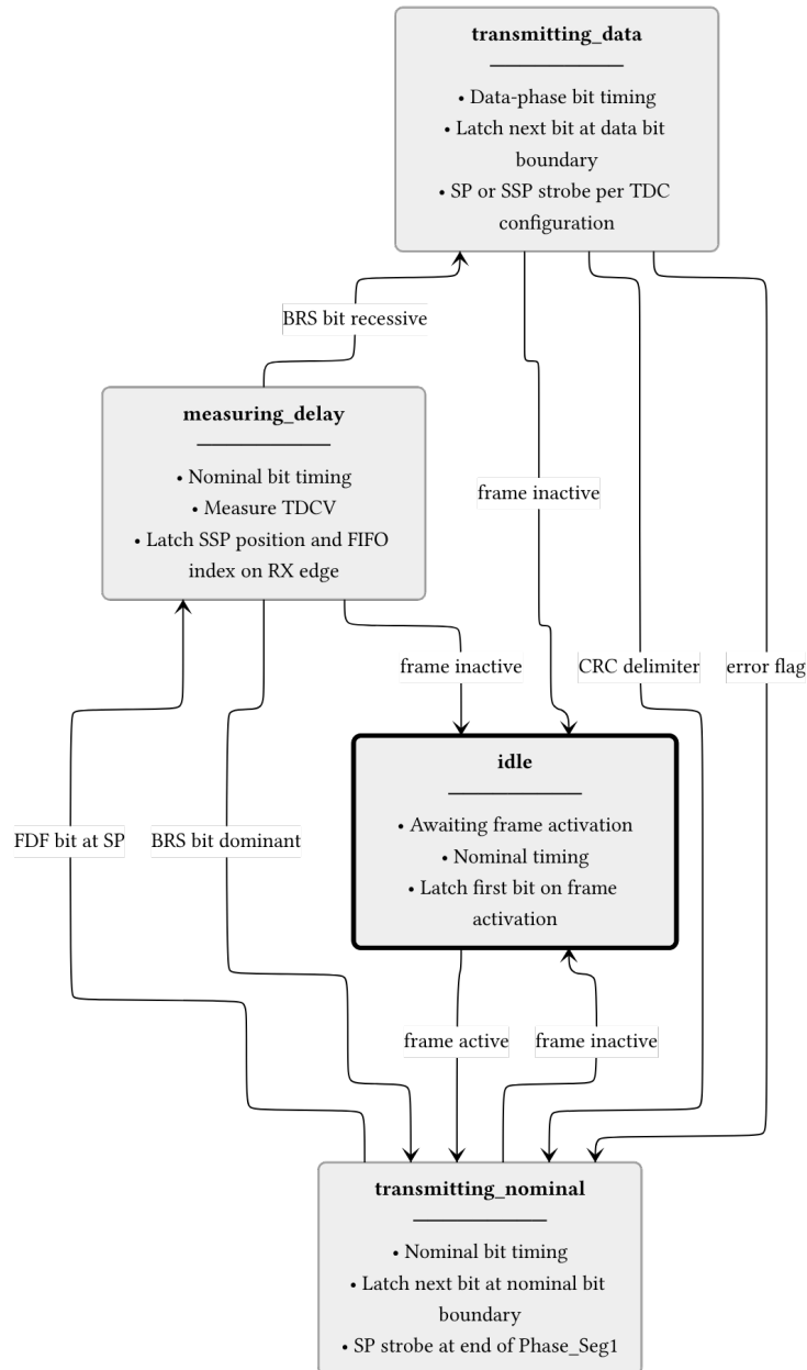
Figure 12: can_pcs_tx FSM. The measuring_delay state is entered on the FDF sample point to measure TDCV (Transmitter Delay Compensation Value, [1] , sec. 7.3.4)]. The BRS bit boundary determines whether data-phase timing is used. All non-idle states return to idle when the frame becomes inactive.
