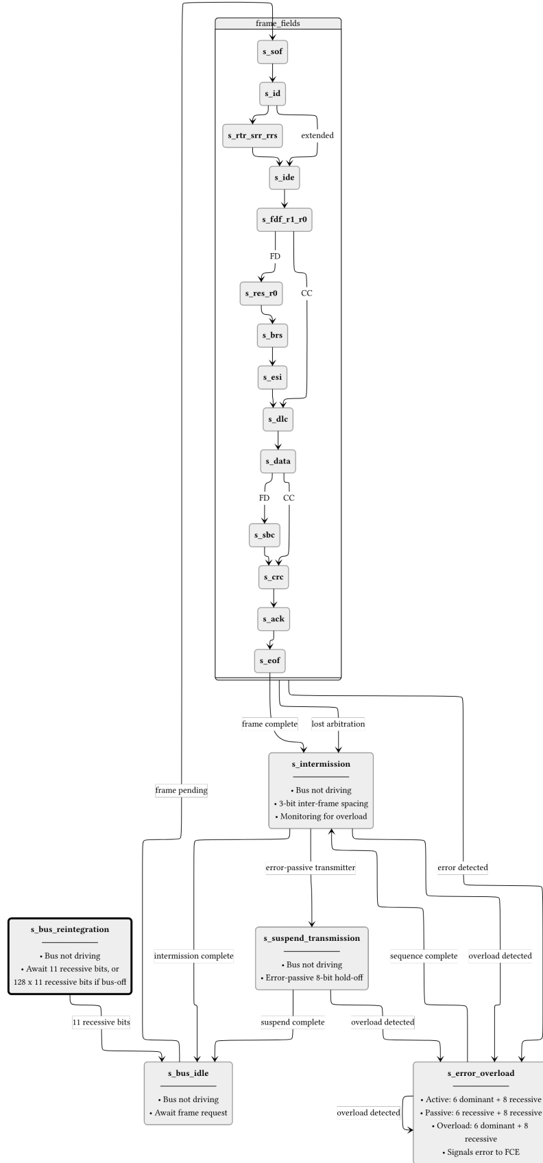
Figure 6: can_mac_fsm_tx FSM with per-field state granularity. Frame-field states (s_sof through s_eof) each handle one protocol field, with bit_count tracking position within the field. After a successful frame or arbitration loss the FSM passes through s_intermission before returning to s_bus_idle. Detected errors branch to s_error_overload, which drives either an active (dominant) or passive (recessive) error flag depending on FCE status. The dashed box groups the frame-field states for clarity.
