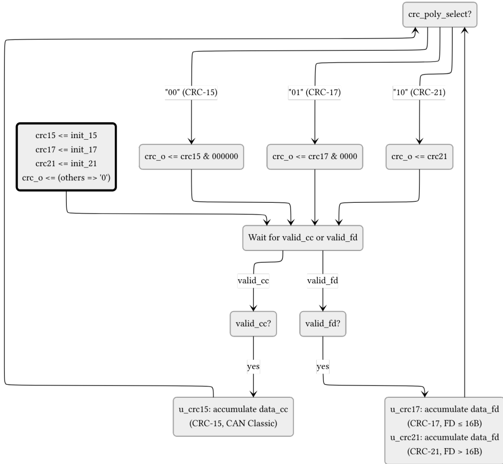
Figure 9: can_mac_crc data path diagram. Three parallel gen_crc instances accumulate continuously: data_cc drives CRC-15 via valid_cc , while data_fd drives both CRC-17 and CRC-21 via valid_fd . The output register selects the active engine result based on crc_poly_select and left-aligns it to 21 bits. The external rst signal reinitializes all three engines and the output register.
