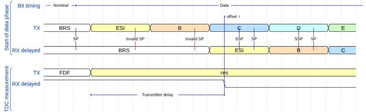
Figure 7: Transmitter Delay Compensation (TDC). The loop delay t_{loop} is measured on the first data-phase bit and used to position the SSP at t_{SSP} = t_{TDC\_offset} + t_{measured} .
