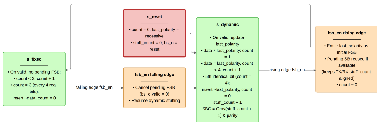
Figure 14: can_mac_bs operating in dynamic and fixed stuffing modes. A pending dynamic stuff bit at the rising edge of fbs_en is promoted to the initial FSB rather than suppressed.
