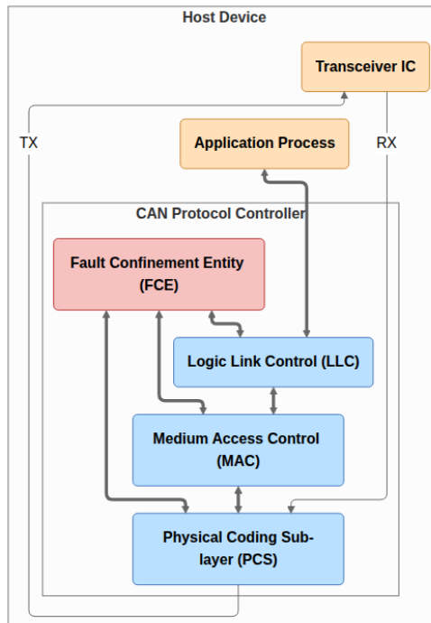
Figure 3: CAN node.
