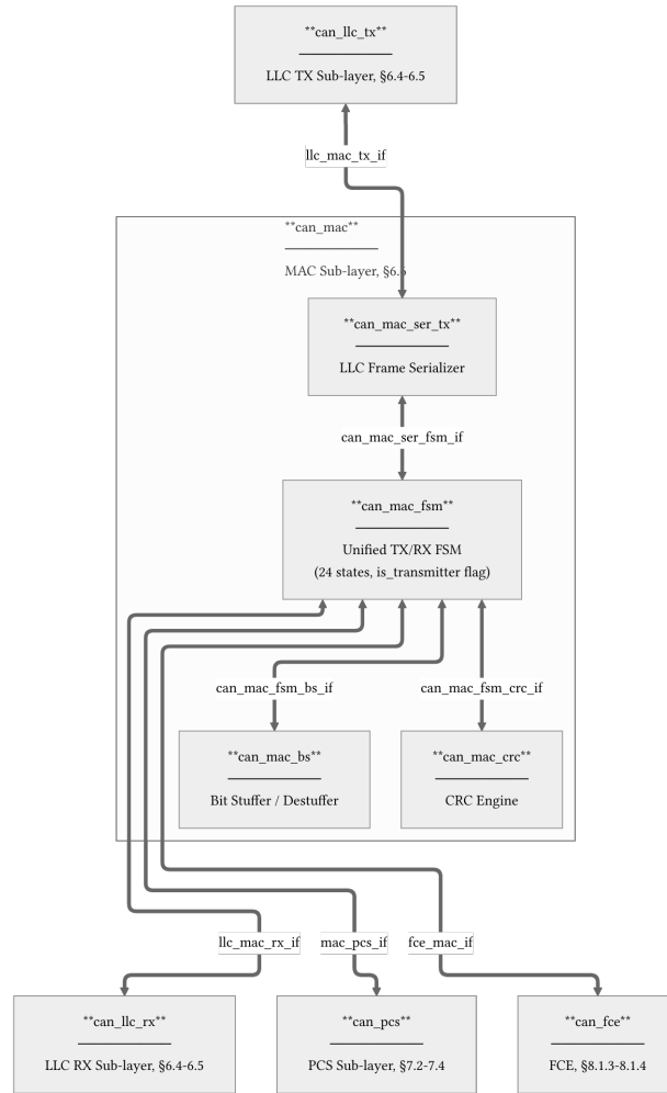
Figure 11: can_mac architecture showing the unified can_mac_fsm and its internal submodules. The FSM instantiates one can_mac_ser_tx serializer, one can_mac_bs bit stuffer, and one can_mac_crc CRC engine, shared across TX and RX modes. Internal interface definitions are provided for can_mac_ser_fsm_if (Table ??), can_mac_fsm_bs_if (Table ??), and can_mac_fsm_crc_if (Table ??).
