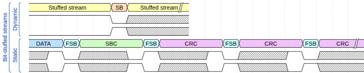
Figure 7: Dynamically and statically bit-stuffed stream examples. In frame fields encoded with dynamic bit-stuffing an opposite polarity stuff bit (SB) is inserted after five consecutive same-polarity bits. In frame fields encoded with static bit-stuffing (SBC and CRC in FD frames) a fixed stuff bit (FSB) is inserted after each fourth bit. A FSB is also inserted before the first bit of the SBC field.
