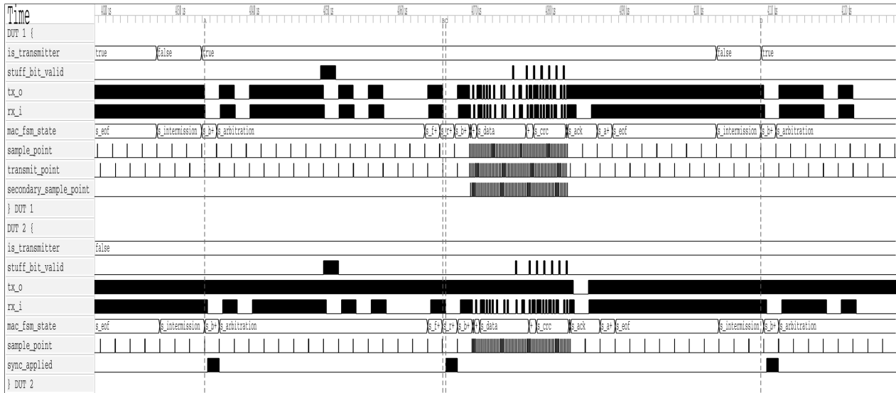
Figure 17: REQ-009. Two-node simulation of a complete FD frame. DUT 1 is the transmitter ( is_transmitter = true ), DUT 2 the receiver. mac_fsm_state traces show the full frame-field sequence from s_arbitration through s_eof ; secondary_sample_point pulses on DUT 1 confirm TDC is active during the data phase; sync_applied pulses on DUT 2 show receiver soft-synchronisation events. After EOF both nodes traverse s_intermission and the sample-point counter accumulates 11 consecutive recessive bits, producing the idle condition and completing bus re-integration (REQ-009).
