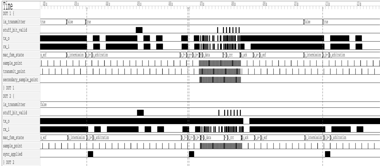
Figure 19: Two-node simulation of a complete FD frame, showing the full FSM field sequence on both transmitter and receiver from s_arbitration through bus re-integration.
