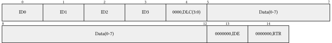
Figure 3: Current LLC frame format (15 bytes). ID byte encoding is defined in Table 5.
