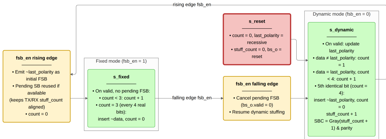
Figure 15: can_mac_bs (two modes). Dynamic mode counts consecutive identical bits and emits an inverse stuff bit on the 5th ( count = 4 ), updating the Gray-coded SBC. Fixed mode is entered on the rising edge of fsb_en , which immediately emits the initial FSB. Thereafter one FSB is emitted every 4 real bits ( count = 3 ). The falling edge of fsb_en cancels any pending FSB and returns to dynamic mode. stuff_count and the SBC output are maintained continuously across both modes.
