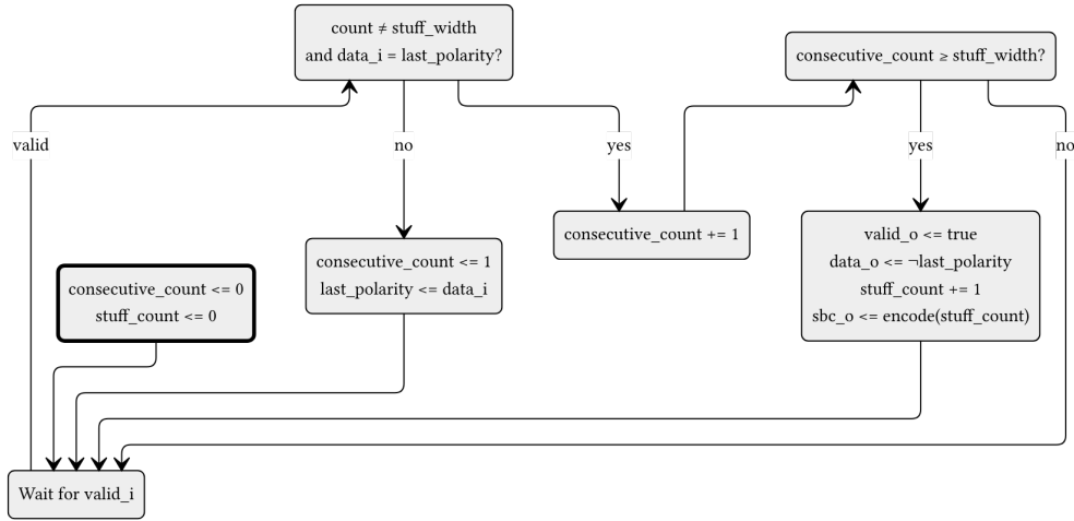
Figure 9: can_mac_bs data path diagram. When valid and data = last_polarity , consecutive_count increments. Otherwise it restarts at 1 with last_polarity updated to data . When consecutive_count reaches stuff_width (5 in dynamic mode, 4 in fixed mode), valid and inverted data are driven and stuff_count increments. The to_gray() + calc_parity() block encodes stuff_count into the stuff_bit_count output. The external rst signal resets consecutive_count and stuff_count to zero. The fixed_bit_stuffing_en signal selects between dynamic and fixed modes. All outputs are registered.
