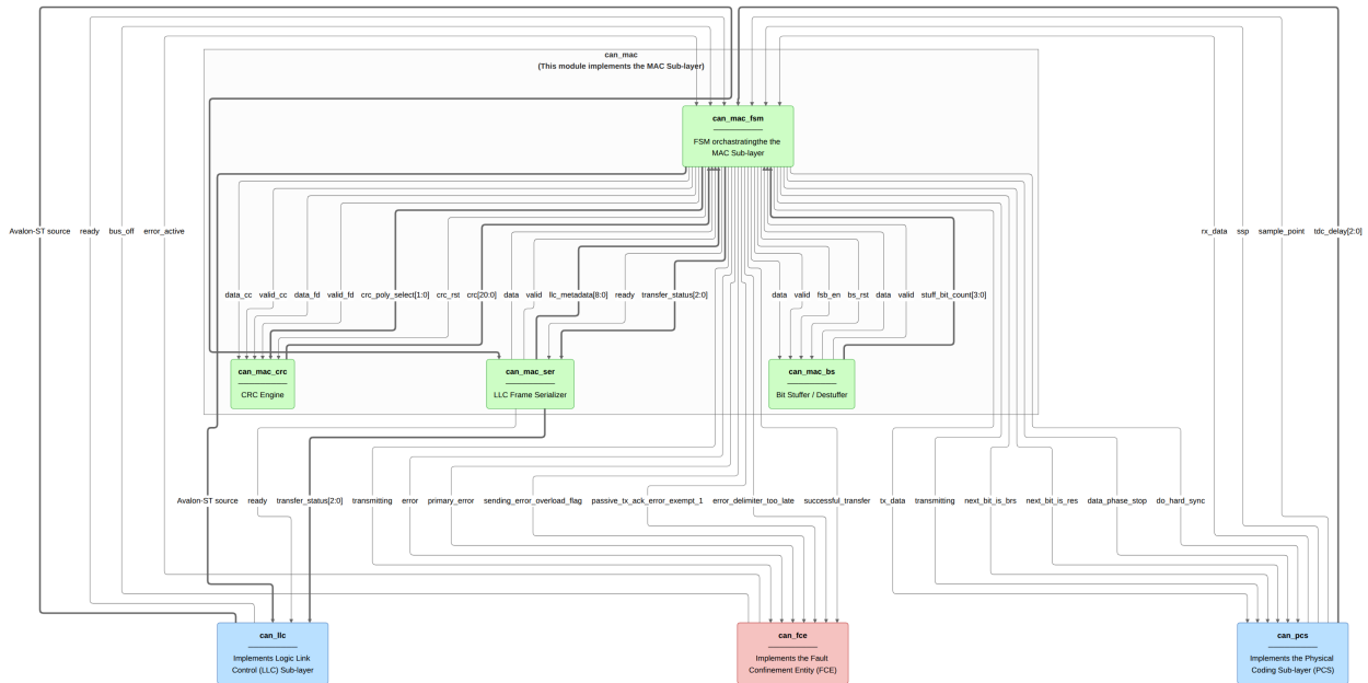
Figure 10: ‘can_mac’ architecture. Individual signals are shown on each directed edge. MAC-internal connections: ‘can_mac_ser’ feeds the serial bit stream and ‘llc_metadata’ to ‘can_mac_fsm’; ‘can_mac_bs’ accepts ‘data/valid/fsb_en’ and returns stuffed ‘data/valid’ plus the Gray-coded ‘stuff_bit_count’ for the SBC field; ‘can_mac_crc’ receives the dual CC/FD bit feeds and returns the running ‘crc[20:0]’ digest. External connections: ‘can_llc’ connects to the MAC on both TX (‘tx_llc_i/o’ via the serializer) and RX (‘rx_llc_i/o’ via the FSM); bit-level timing to ‘can_pcs’ (‘tx_data’, ‘rx_data’, sample-point strobes); fault-confinement events to/from ‘can_fce’ (‘error_active’, ‘bus_off’).
