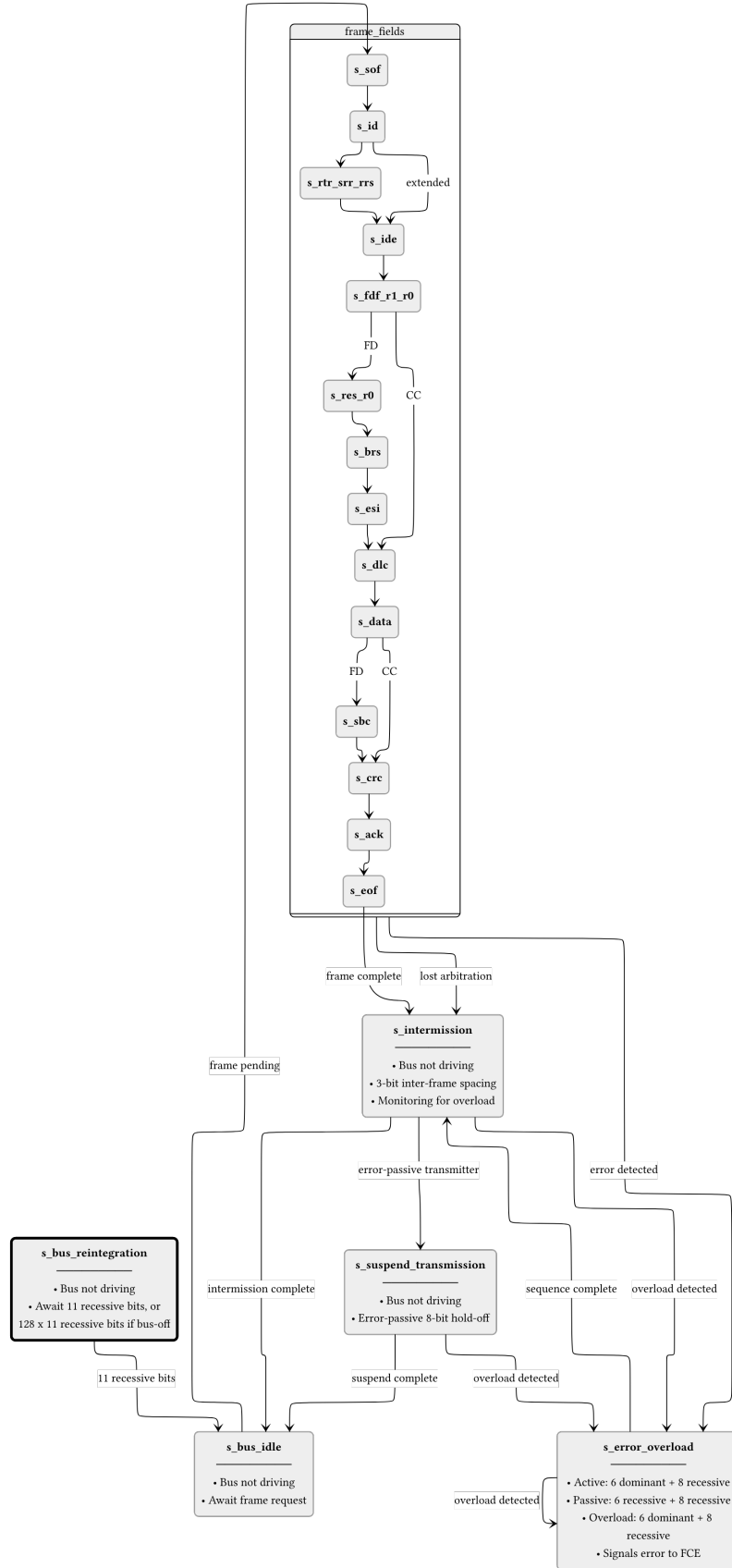
Figure 5: can_mac_fsm_tx FSM with per-field state granularity. Frame-field states ( s_{\text{sof}} through s_{\text{eof}} ) each handle one protocol field, with \text{bit\_count} tracking position within the field. After a successful frame or arbitration loss the FSM passes through s_{\text{intermission}} before returning to s_{\text{bus\_idle}} . Detected errors branch to s_{\text{error\_overload}} , which drives either an active (dominant) or passive (recessive) error flag depending on FCE status. The dashed box groups the frame-field states for clarity.
