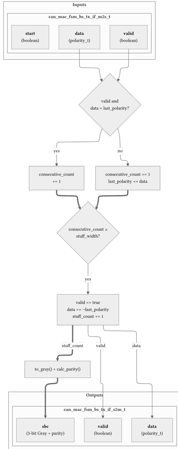
Figure 8: can_mac_bs_tx data path diagram. When valid and data = last_polarity, consecutive_count increments. Otherwise it restarts at 1 with last_polarity updated to data. When consecutive_count reaches stuff_width, valid and inverted data are driven and stuff_count increments. The to_gray() + calc_parity() block encodes stuff_count into the sbc output. The start pulse resets consecutive_count and stuff_count to zero. All outputs are registered.
