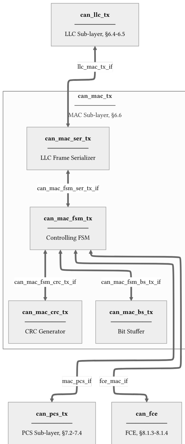
Figure 5: can_mac_tx architecture showing internal component interconnections and external interfaces. Internal interface definitions are provided for can_mac_fsm_ser_tx_if (Table 11), can_mac_fsm_bs_tx_if (Table 12), and can_mac_fsm_crc_tx_if (Table 13).
