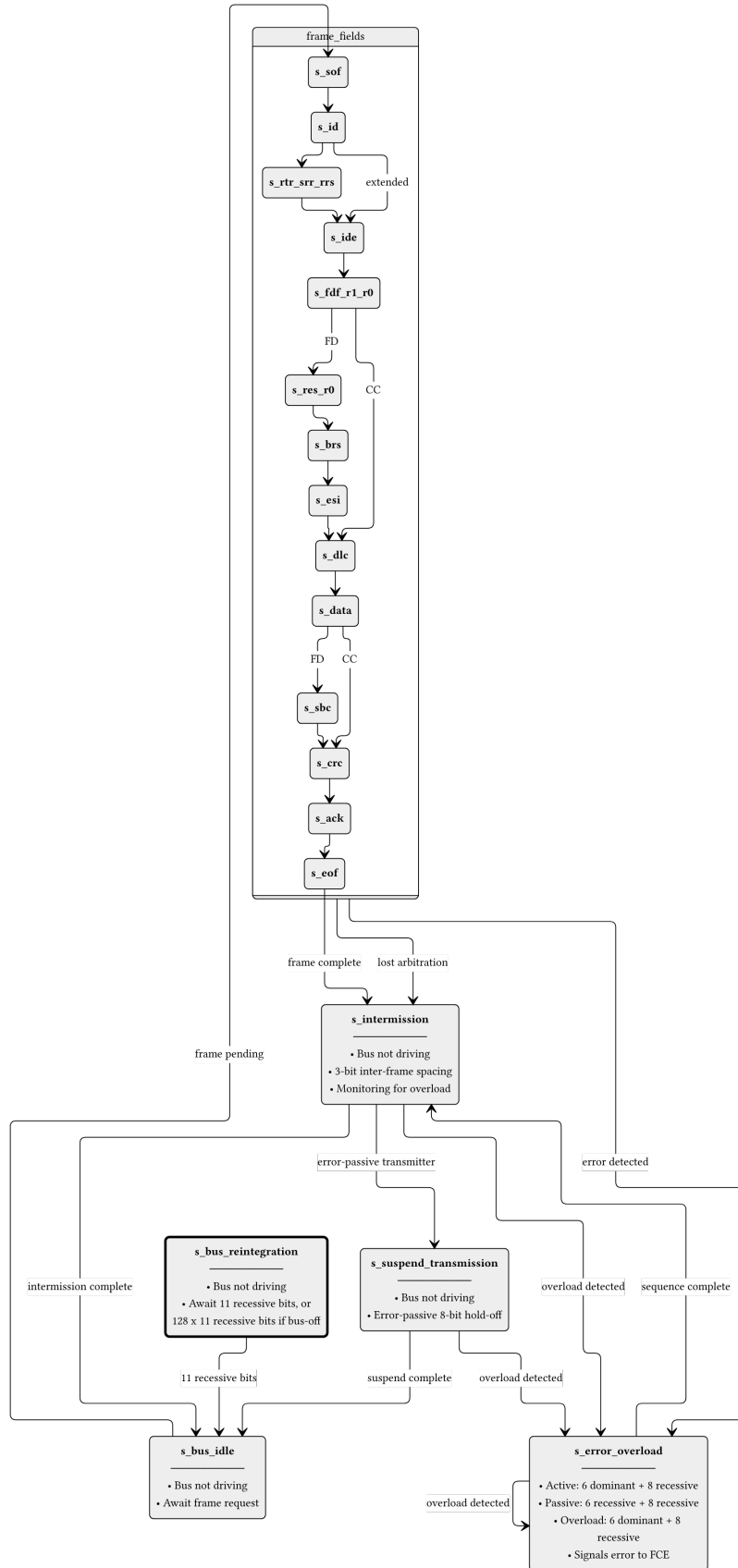
Figure 6: can_mac_fsm_tx FSM with per-field state granularity. Frame-field states ( s_sof through s_eof ) each handle one protocol field, with bit_count tracking position within the field. After a successful frame or arbitration loss the FSM passes through s_intermission before returning to s_bus_idle . Detected errors branch to s_error_overload , which drives either an active (dominant) or passive (recessive) error flag depending on FCE status. The dashed box groups the frame-field states for clarity.
