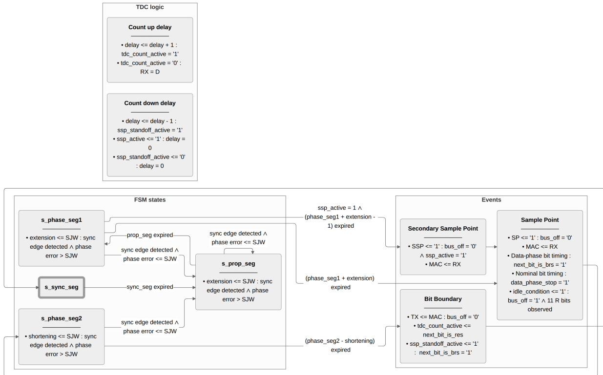
Figure 17: can_pcs FSM implementing CAN node bit timing, synchronization and TDC logic.
