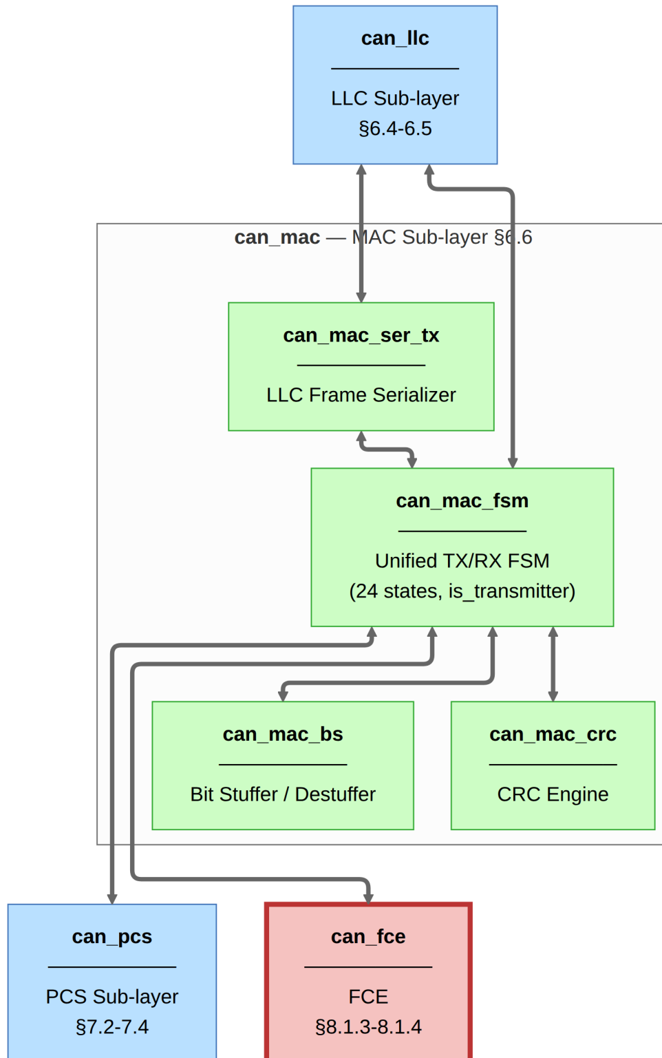
Figure 11: can_mac module topology. Each bidirectional edge represents one or more interface signals between the connected modules. The detailed per-signal breakdown is given in Figure ??.
