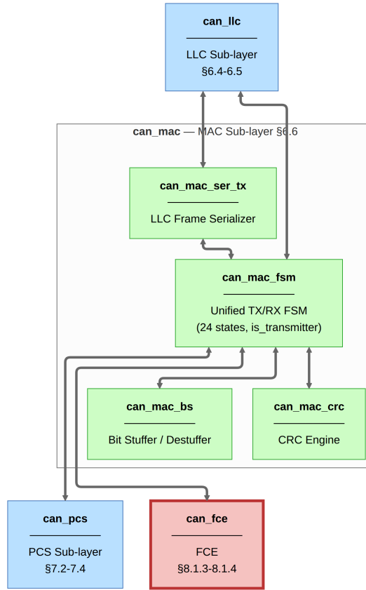
Figure 10: Implementation module decomposition. can_llc provides the Avalon-ST host interface and manages retransmission and acceptance filtering. Inside can_mac , the unified can_mac_fsm handles both TX and RX roles via a single is_transmitter flag, sharing one can_mac_bs bit stuffer and one can_mac_crc engine. can_pcs generates sample-point and SSP strobes. can_fce maintains TEC/REC counters and governs node-state transitions.
