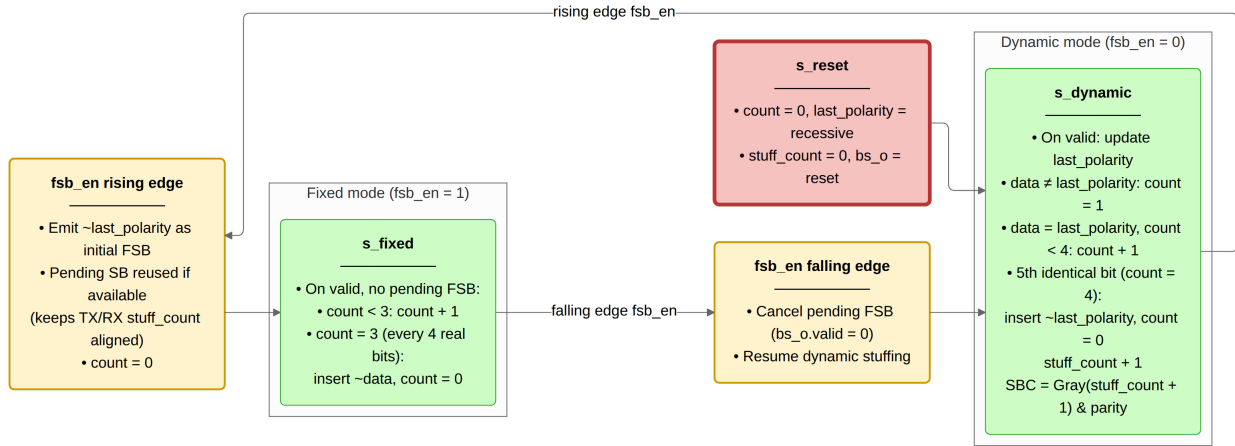
Figure 15: can_mac_bs (2 modes). Dynamic mode counts consecutive identical bits and emits an inverse stuff bit on the 5th (count = 4), updating the Gray-coded SBC. Fixed mode is entered on the rising edge of fsb_en , which immediately emits the initial FSB. Thereafter one FSB is emitted every 4 real bits (count = 3). The falling edge of fsb_en cancels any pending FSB and returns to dynamic mode. stuff_count and the SBC output are maintained continuously across both modes.
