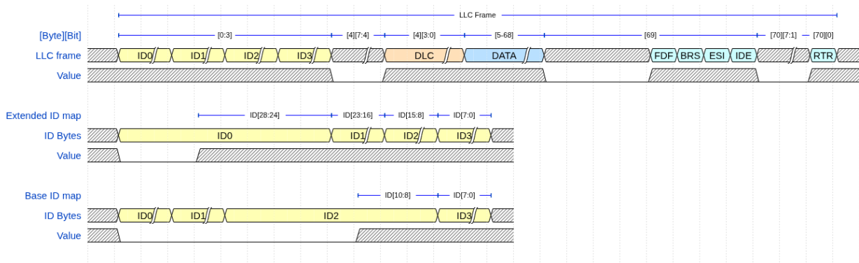
Figure 11: LLC frame format (71 bytes) at the host-MAC interface. Bytes 0-3 encode the identifier. Byte 4 carries the frame-type selector FTFP in bits [7:4] and DLC in bits [3:0]. Bytes 5-68 carry up to 64 data bytes. Byte 69 carries the FDF, BRS, ESI, and IDE control flags. Byte 70 carries RTR in bit 0. The lower rows show the identifier byte mapping: for extended identifiers ID[28:24] are packed into ID0, ID[23:16] into ID1, ID[15:8] into ID2, and ID[7:0] into ID3. For base identifiers ID0 and ID1 are all zeros, ID[10:8] occupies the lower three bits of ID2, and ID[7:0] fills ID3.
