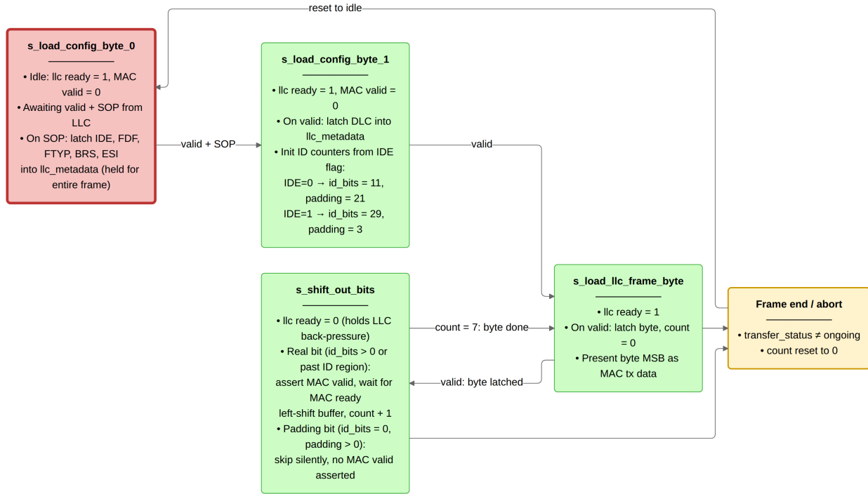
Figure 14: can_mac_ser (4 states). Config bytes carry frame metadata (IDE, FDF, FTYP, BRS, ESI, DLC). These are latched once and held stable for the entire frame. In s_shift_out_bits real ID and data bits are driven one per MAC FSM ready pulse, while unused padding bits in the 32-bit ID field are skipped silently. Any transfer_status != ongoing signal from the MAC FSM returns the serializer to s_load_config_byte_0 from any state.
