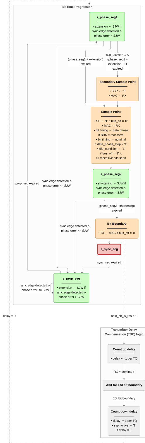
Figure 18: can_pcs operation (ISO 11898-1 sec. 7.2-7.4). Two concurrent-per-TQ blocks are shown alongside the main bit time progression. The bit time progression (center) cycles through s_sync_seg (1 TQ fixed, red reset state), s_prop_seg, s_phase_seg1, and s_phase_seg2 (green). A sync edge detected mid-segment triggers resynchronization: with phase error at most SJW the bit time restarts from s_prop_seg. With larger error s_phase_seg1 is extended or s_phase_seg2 shortened by SJW. Three bus events (orange) mark the IO moments within each bit time: SSP samples rx_i one TQ before the SP when ssp_active is set. The SP samples rx_i, switches to data-phase timing on a recessive BRS, or restores nominal timing on data_phase_stop, and pulses idle_condition when bus_off is asserted and 11 consecutive recessive bits have been seen. The bit boundary drives tx_o. The TDC pipeline (right) runs concurrently per TQ, transmitting only. A dashed edge from the bit boundary activates it when next_bit_is_res: recessive TQs are counted until the TX-to-RX echo arrives, then at the ESI bit boundary a countdown begins and ssp_active is set when the count reaches zero.
