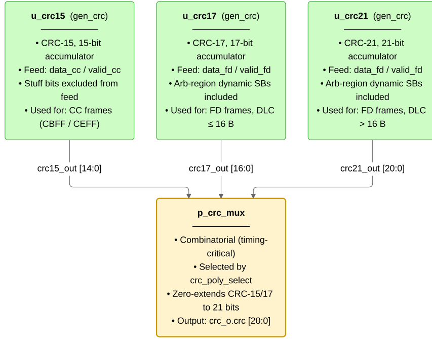
Figure 16: can_mac_crc dataflow. Three gen_crc instances accumulate in parallel on every clock: u_crc15 is fed by data_cc/valid_cc (CC bit stream, stuff bits excluded). u_crc17 and u_crc21 are both fed by data_fd/valid_fd (FD bit stream, dynamic stuff bits included in the arbitration region). The combinatorial mux p_crc_mux selects the active engine result based on crc_poly_select and zero-extends it to the common 21-bit output. reset_i reinitializes all three engines simultaneously.
