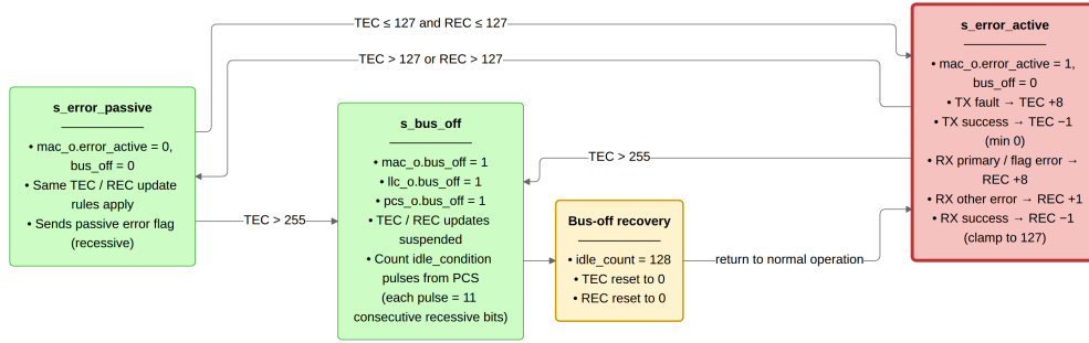
Figure 17: can_fce FSM (ISO 11898-1 sec. 8.1.4.4, Figure 43). s_error_active is the initial state after reset_i or llc_i.normal_mode . When TEC exceeds 127 or REC exceeds 127 the FCE moves to s_error_passive , clearing mac_o.error_active . If TEC exceeds 255 from either active or passive state, the FCE enters s_bus_off , asserting bus_off to the MAC, LLC, and PCS. Recovery counts 128 idle_condition pulses from the PCS (each pulse represents 11 consecutive recessive bits). On the 128th pulse TEC and REC are reset to zero and the FSM returns to s_error_active .
