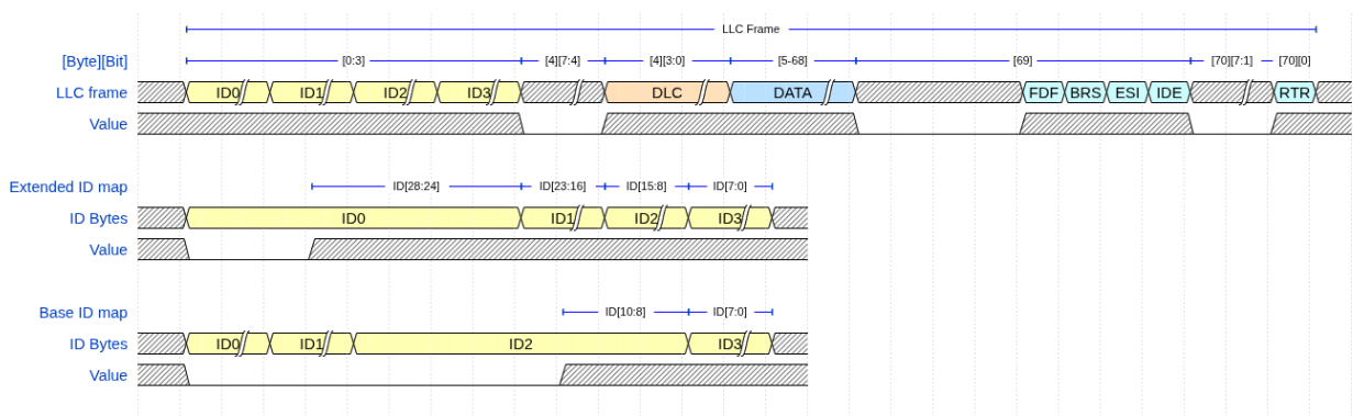
Figure 11: LLC frame format (71 bytes) at the host-LLC interface. Bytes 0-3 carry the identifier as four bytes ID0-ID3. Byte 4 bits [7:4] carry the frame-type selector FTYP and bits [3:0] carry DLC. Bytes 5-68 carry up to 64 data bytes. Byte 69 bits [3:0] carry the control flags FDF, BRS, ESI, and IDE, with bits [7:4] reserved. Byte 70 bit [0] carries RTR, with bits [7:1] reserved. The lower two rows show the identifier byte mapping: for extended 29-bit identifiers ID[28:24] is packed into the lower five bits of ID0, ID[23:16] into ID1, ID[15:8] into ID2, and ID[7:0] into ID3. For base 11-bit identifiers, ID0 and ID1 are all zeros, ID[10:8] occupies the lower three bits of ID2, and ID[7:0] fills ID3.
