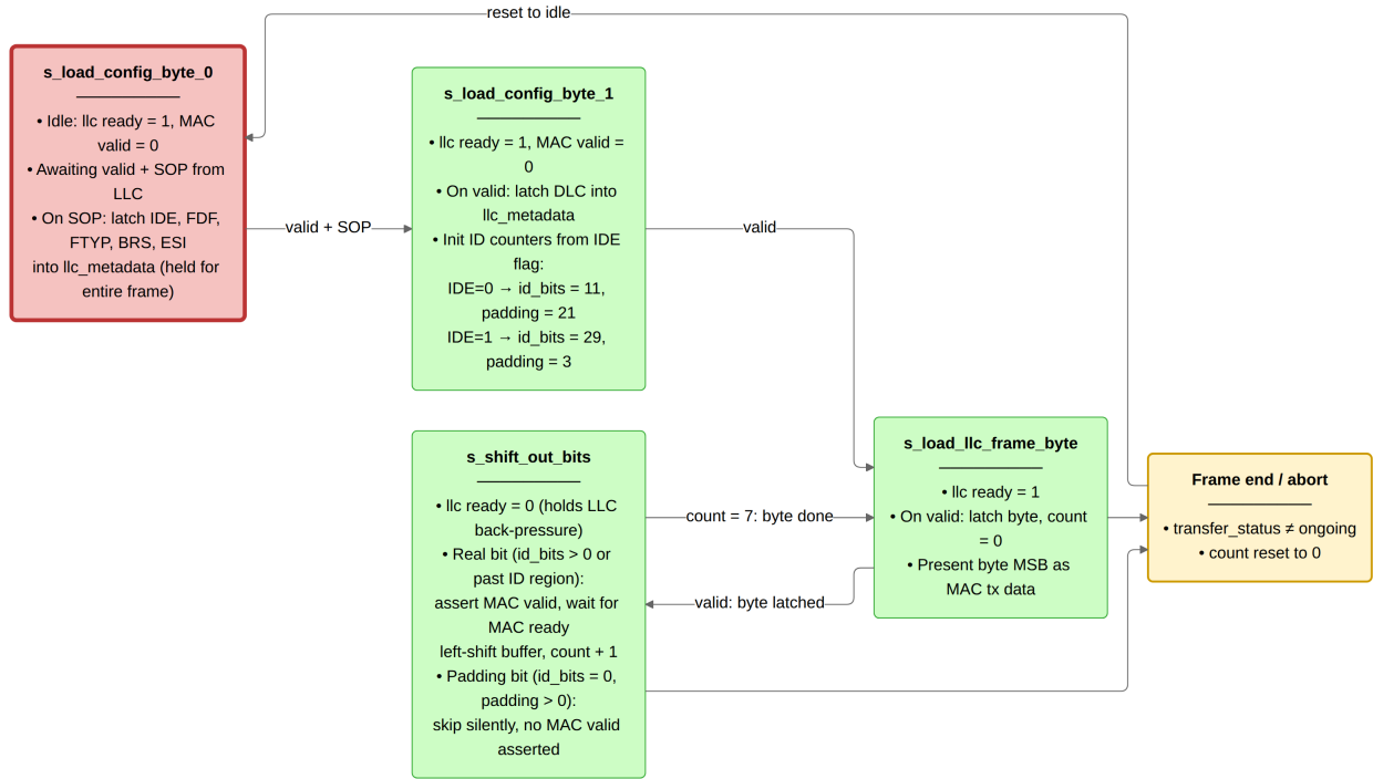
Figure 14: can_mac_ser (four states). Config bytes carry frame metadata (IDE, FDF, FTYP, BRS, ESI, DLC). These are latched once and held stable for the entire frame. In s_shift_out_bits real ID and data bits are driven one per MAC FSM ready pulse, while unused padding bits in the 32-bit ID field are skipped silently. Any transfer_status ≠ ongoing signal from the MAC FSM returns the serializer to s_load_config_byte_0 from any state.
