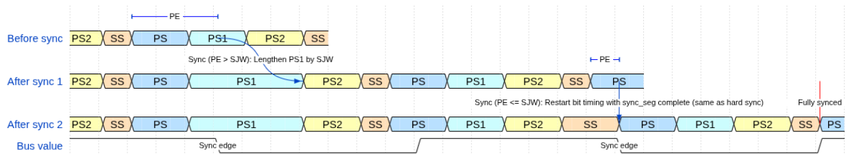
Figure 6: Resynchronization over two successive sync edges (REQ-027). The phase error (PE) is the displacement between the received recessive-to-dominant edge and the start of SYNC_SEG. When PE exceeds SJW, PHASE_SEG1 is lengthened by exactly SJW quanta (After sync 1), moving the sample point forward by SJW. When PE is at most SJW, bit timing is restarted from SYNC_SEG on the incoming edge - equivalent to a hard synchronization - absorbing the full phase error in one step (After sync 2). After two such corrections the node is fully synchronized to the transmitter.
