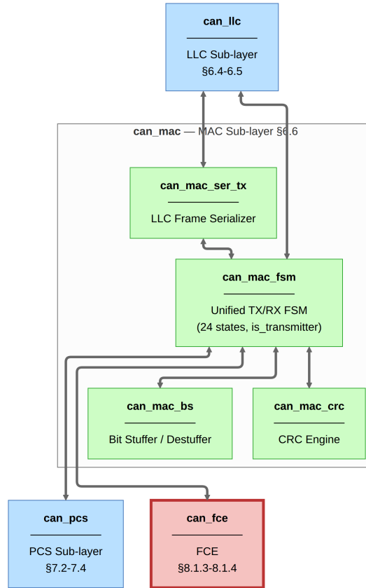
Figure 10: Implementation module decomposition. can_llc provides the Avalon-ST host interface and manages retransmission and acceptance filtering. Inside can_mac , the unified can_mac_fsm handles both TX and RX roles via a single is_transmitter flag, sharing one can_mac_bs bit stuffer and one can_mac_crc engine. can_pcs generates sample-point and SSP strobes. can_fce maintains TEC/REC counters and governs node-state transitions.
