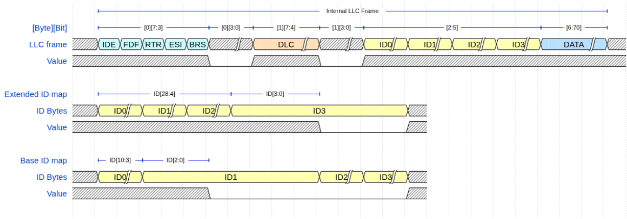
Figure 9: Internal LLC frame format at the can_mac_ser input. Byte 0 bits [7:3] pack the five frame-type flags IDE, FDF, FTYP (RTR), ESI, and BRS. Bits [2:0] of byte 0 and [3:0] of byte 1 are reserved zeros. Byte 1 bits [7:4] carry DLC. Bytes 2-5 carry the 32-bit identifier as four bytes ID0-ID3, MSB-first. Bytes 6-70 carry up to 64 data bytes. The lower two rows show the identifier byte mapping: for extended 29-bit identifiers ID[28:4] is packed across the first three ID bytes and ID[3:0] into ID3. For base 11-bit identifiers, ID[10:3] fills ID0, ID[2:0] occupies the upper three bits of ID1, and the remaining bits of ID1 through ID3 are all zeros.
