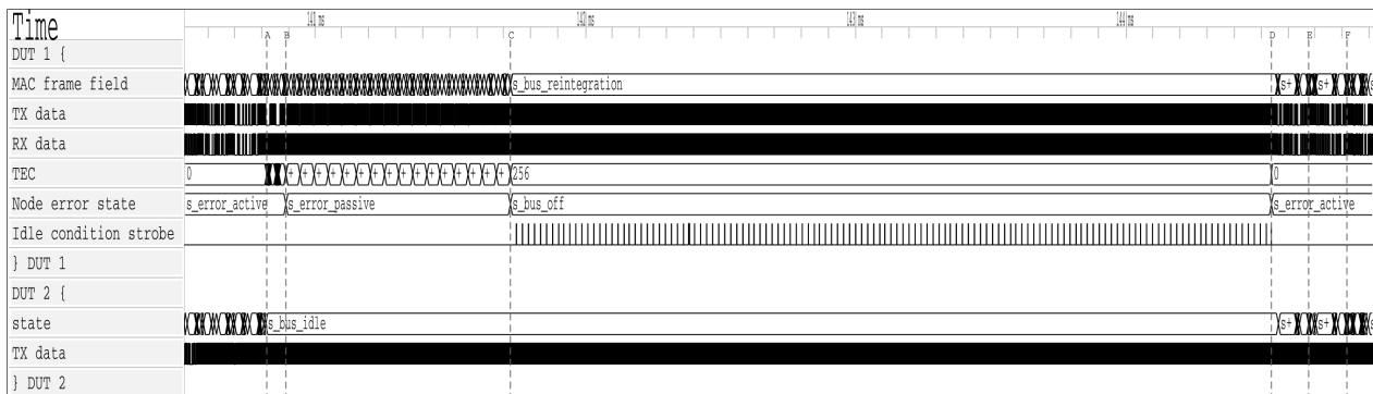
Figure 24: Bus-off recovery in can_mac_pcs_fce_tb. DUT 1 transmits the first active error flag at A. At B, TEC reaches 128 and the node transitions to error passive. At C, TEC reaches 256 and the node enters bus off. The FCE counts 128 idle condition strobes from the PCS and restores s_error_active at D. At E and F, DUT 2 acknowledges the first two frames transmitted after recovery.
