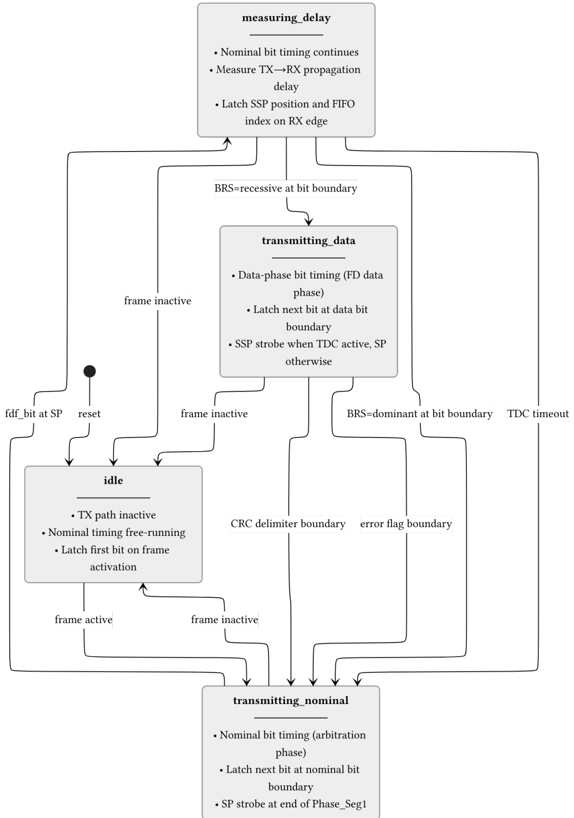
Figure 7: PCS TX FSM state transitions. The measuring_delay state is entered on the FDF sample point to measure the TX-to-RX propagation delay for TDC. The BRS bit boundary determines whether data-phase timing is used. All non-idle states return to idle when the frame becomes inactive.
