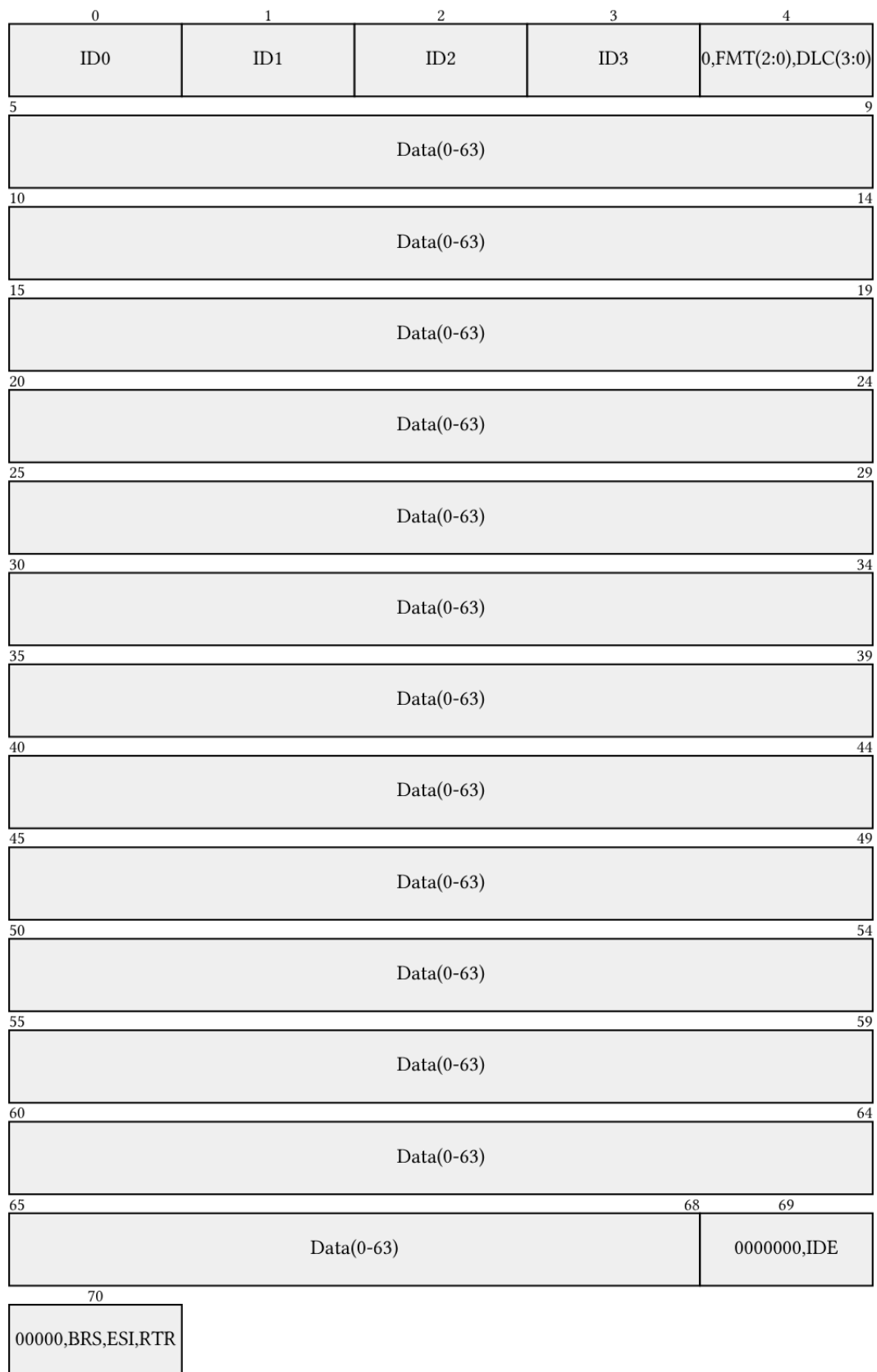
Figure 3: Maximum length revised LLC Frame format with FD support.
