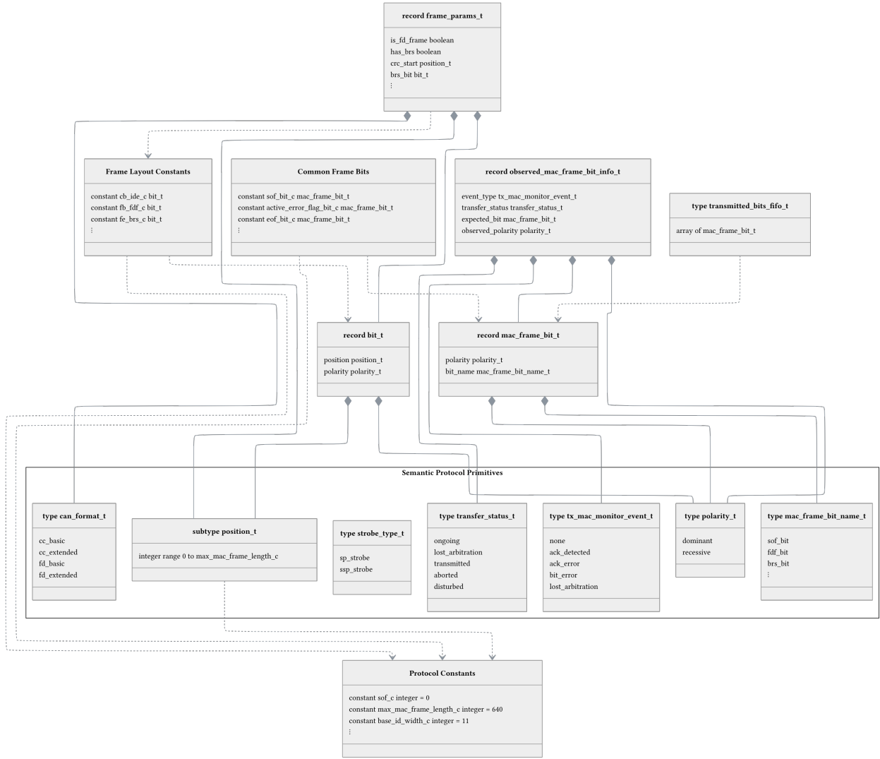
Figure 4: Type and constant hierarchy. Protocol constants derived from ISO 11898-1 form the root of the hierarchy, from which frame layout constants, type constraints, and composite record types are derived. The TX Monitoring namespace groups the types used by get_observed_mac_frame_bit_info() to classify bus events on each sample-point strobe and support TDC-delayed bit comparison via the transmitted-bits FIFO.
