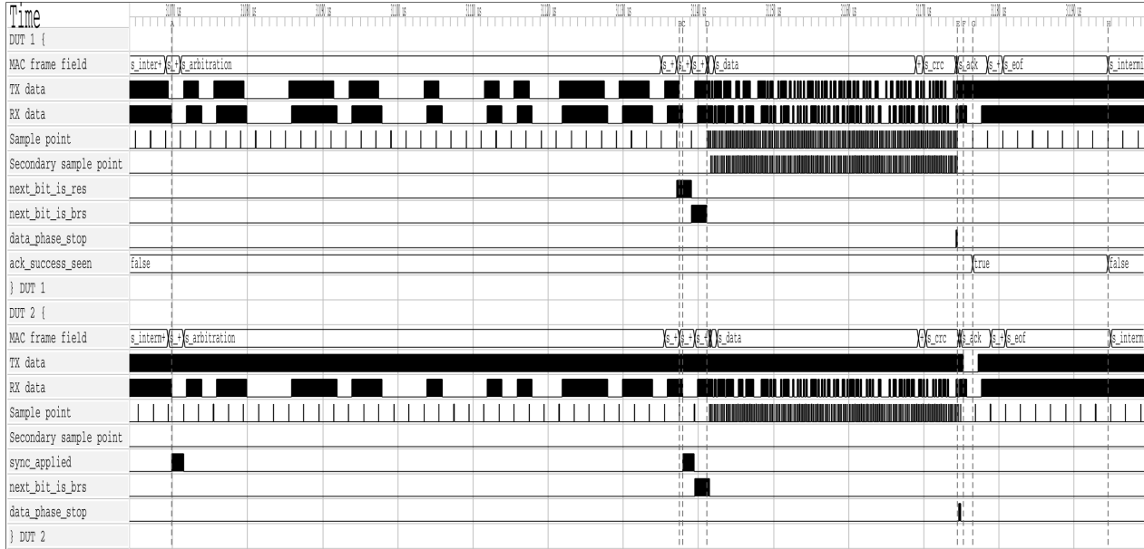
Figure 19: Two-node simulation of a complete FD frame transmission in can_mac_pcs_fce_tb. DUT 2 does hard sync on SOF at A. DUT 1 does the TDC measurement between B and C. Bot nodes switch to data phase bit timing at the BRS sample point at D. DUT 1 switches back to nominal bit timing at the CRC delimiter sample point at E. DUT 2 drives the ACK slot dominant at F, DUT 1 samples the dominant ACK at G and latches ack_success_seen. Transmission ends at H
