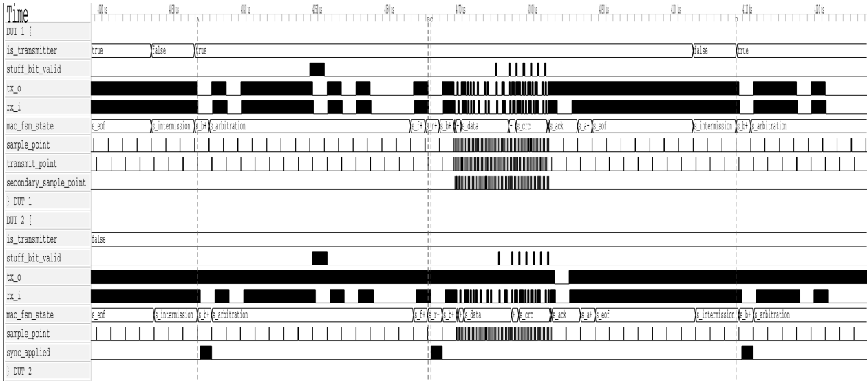
Figure 19: REQ-009 . Two-node simulation of a complete FD frame. DUT 1 is the transmitter ( is_transmitter = true ), DUT 2 the receiver. mac_fsm_state traces show the full frame-field sequence from s_arbitration through s_eof . secondary_sample_point pulses on DUT 1 confirm TDC is active during the data phase. sync_applied pulses on DUT 2 show receiver resynchronization events. After EOF both nodes traverse s_intermission and the sample-point counter accumulates 11 consecutive recessive bits, producing the idle condition and completing bus re-integration ( REQ-009 ).
