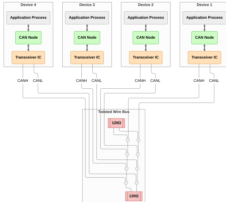
Figure 1: CAN bus consisting of four CAN nodes connected via a shared differential two-wire bus. Each node contains a CAN protocol controller and transceiver IC. Termination resistors at each end of the bus prevent signal reflections.
