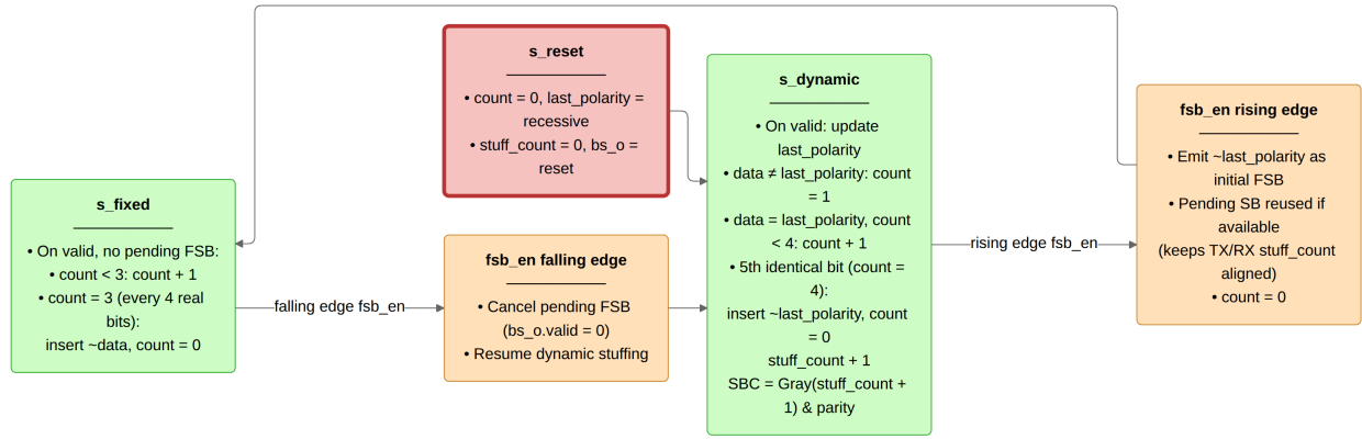
Figure 15: can_mac_bs (two modes). Dynamic mode counts consecutive identical bits and emits an inverse stuff bit on the 5th (count = 4), updating the Gray-coded SBC. Fixed mode is entered on the rising edge of fsb_en, which immediately emits the initial FSB. Thereafter one FSB is emitted every 4 real bits (count = 3). The falling edge of fsb_en cancels any pending FSB and returns to dynamic mode. stuff_count and the SBC output are maintained continuously across both modes.
