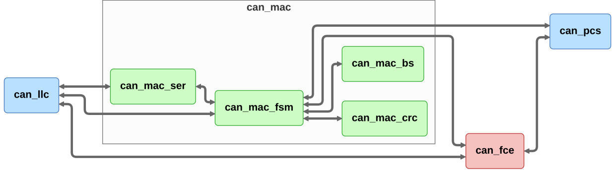
Figure 10: Implementation module decomposition. can_llc provides the Avalon-ST host interface and manages retransmission and acceptance filtering. Inside can_mac , the unified can_mac_fsm handles both TX and RX roles via a single is_transmitter flag, sharing one can_mac_bs bit stuffer and one can_mac_crc engine. can_pcs generates sample-point and SSP strobes. can_fce maintains TEC/REC counters and governs node-state transitions.
