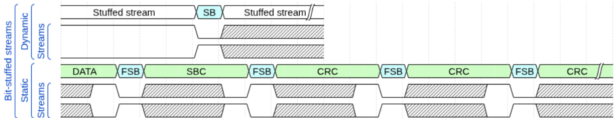
Figure 6: Dynamically and statically bit-stuffed stream examples. In frame fields encoded with dynamic bit-stuffing an opposite polarity stuff bit (SB) is inserted after five consecutive same-polarity bits. In frame fields encoded with static bit-stuffing (SBC and CRC in FD frames) a fixed stuff bit (FSB) is inserted after each fourth bit. A FSB is also inserted before the first bit of the SBC field.
