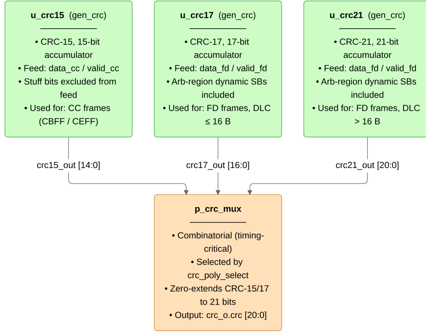
Figure 15: can_mac_crc dataflow with three parallel CRC engines. The output mux is combinatorial to satisfy the \text{ISO IPT} \leq 2 t_q constraint at minimum prescaler.
