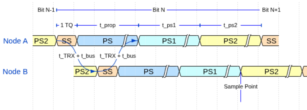
Figure 5: CAN bit time structure showing the four segments (SS, PS, PS1, PS2), the sample point, and propagation delays on a two-node bus.
