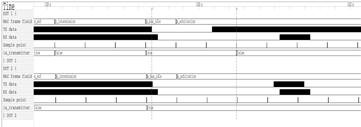
Figure 23: Arbitration loss in can_mac_pcs_fce_tb . Both nodes enter s_arbitration as transmitters at A. DUT 1 loses arbitration at B after transmitting recessive and sampling dominant, and continues as receiver with is_transmitter cleared.
