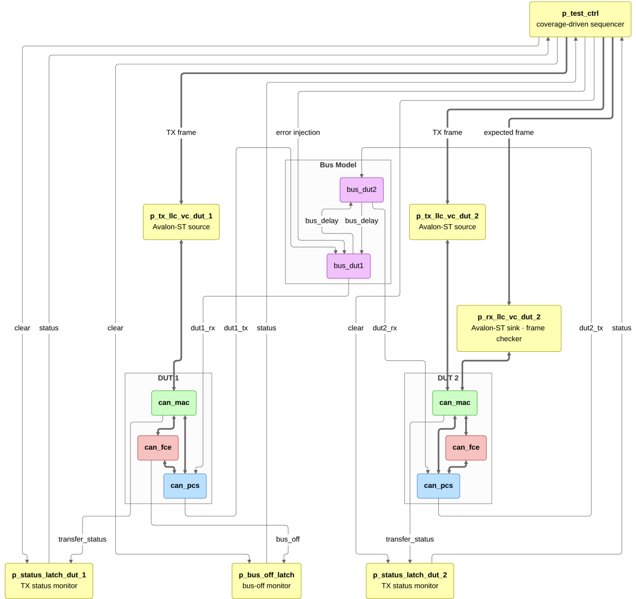
Figure 19: can_mac_pcs_fce_tb integration testbench. Two can_mac_pcs_fce instances connect through a dominant-wins bus model. Avalon-ST VCs drive and sample the MAC interfaces. p_test_ctrl sequences test stimuli, injects bit errors via dut_1_rx_recessive , and reads pass/fail status from the TX-status and bus-off monitors.
