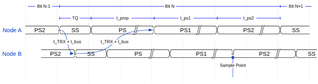
Figure 5: CAN nominal bit time structure. One bit consists of SYNC_SEG (1 TQ), PROP_SEG, PHASE_SEG1, and PHASE_SEG2. The sample point (SP) sits at the PHASE_SEG1/PHASE_SEG2 boundary. In the CAN FD data phase the total bit period is shorter but the four-segment structure is preserved with independently configured values.
