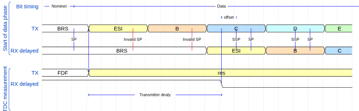
Figure 7: Transmitter Delay Compensation (TDC). At high data-phase bit rates the sum of bus propagation and transceiver delays ( t_{\text{loop}} ) may exceed one nominal bit time, causing the echo of a driven bit to arrive too late for the standard sample point. TDC measures this loop delay during the first data-phase bit and positions the Secondary Sample Point (SSP) at offset t_{\text{SSP}} = t_{\text{TDC\_offset}} + t_{\text{measured}} , so that each transmitted bit is verified against its bus echo at the correct moment. The SSP replaces the nominal SP for bit-error monitoring throughout the data phase [1, Sec. 7.3.4].
