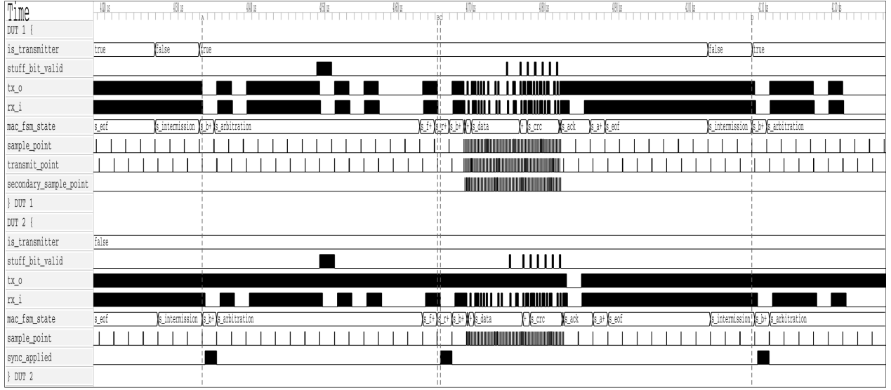
Figure 18: REQ-009 . Two-node simulation of a complete FD frame. DUT 1 is the transmitter ( is_transmitter = true ), DUT 2 the receiver. mac_fsm_state traces show the full frame-field sequence from s_arbitration through s_eof ; secondary_sample_point pulses on DUT 1 confirm TDC is active during the data phase; sync_applied pulses on DUT 2 show receiver soft-synchronisation events. After EOF both nodes traverse s_intermission and the sample-point counter accumulates 11 consecutive recessive bits, producing the idle condition and completing bus re-integration ( REQ-009 ).
