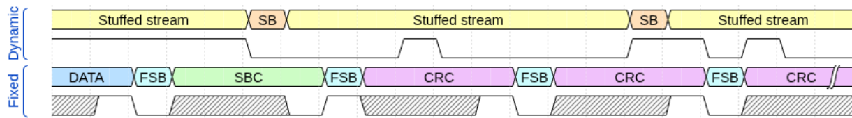
Figure 8: Dynamic and fixed bit-stuffing examples. In frame fields encoded with dynamic bit-stuffing an opposite polarity stuff bit (SB) is inserted after five consecutive same-polarity bits. In frame fields encoded with fixed bit-stuffing (SBC and CRC in FD frames) a fixed stuff bit (FSB) is inserted after each fourth bit. A FSB is also inserted before the first bit of the SBC field.
