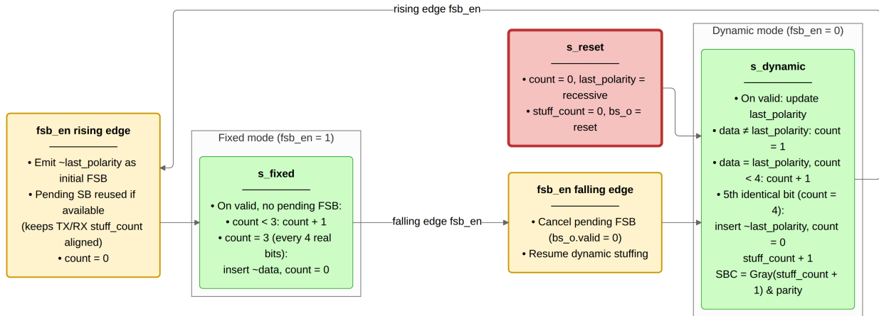
Figure 14: can_mac_bs (2 modes). Dynamic mode counts consecutive identical bits and emits an inverse stuff bit on the 5th (count = 4), updating the Gray-coded SBC. Fixed mode is entered on the rising edge of fsb_en, which immediately emits the initial FSB. Thereafter one FSB is emitted every 4 real bits (count = 3). The falling edge of fsb_en cancels any pending FSB and returns to dynamic mode. stuff_count and the SBC output are maintained continuously across both modes.
