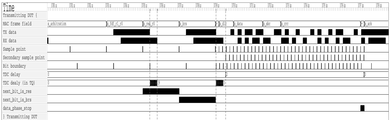
Figure 22: Dual bit rate switching and TDC measurement in can_mac_pcs_fce_tb . At A, the PCS begins counting the transceiver loopback delay in TQ increments. At B, the transmitted bit arrives on RX and the count stops at 19 TQ. At C, the first data-phase bit (ESI) is transmitted and the measured delay is counted down. When the countdown terminates at D, the SSP strobe activates and the TDC delay of 2 is signaled to the MAC. next_bit_is_res and next_bit_is_brs control the measurement window. data_phase_stop signals the end of the data phase.
