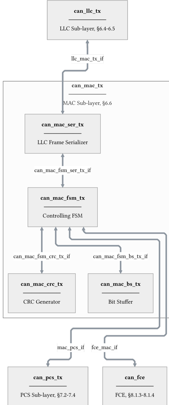
Figure 5: MAC TX layer architecture showing internal component interconnections and external interfaces (LLC, PCS, FCE). Internal interface definitions are provided for can_mac_fsm_ser_tx_if (Table 11), can_mac_fsm_bs_tx_if (Table 12), and can_mac_fsm_crc_tx_if (Table 13).
