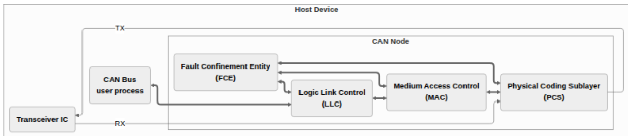
Figure 3: CAN node.
