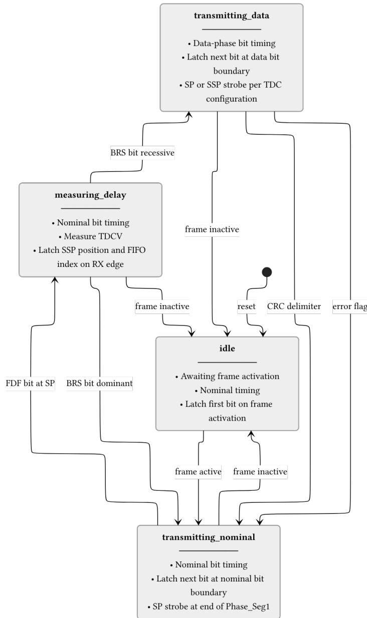
Figure 8: can_pcs_tx FSM. The measuring_delay state is entered on the FDF sample point to measure TDCV (Transmitter Delay Compensation Value, [1], sec. 7.3.4). The BRS bit boundary determines whether data-phase timing is used. All non-idle states return to idle when the frame becomes inactive.
