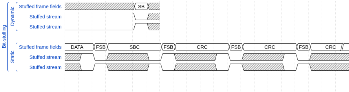
Figure 6: Dynamic bit stuffing: five consecutive bits of the same polarity trigger insertion of one complement stuff bit (S). The receiver detects and removes the stuff bit. A sixth consecutive same-polarity bit is a stuff error.
