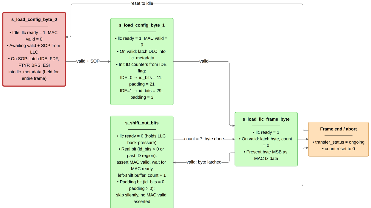
Figure 13: can_mac_ser FSM (four states) serializing the internal LLC frame to the MAC bit stream. Unused padding bits in the 32-bit ID field are skipped silently.
