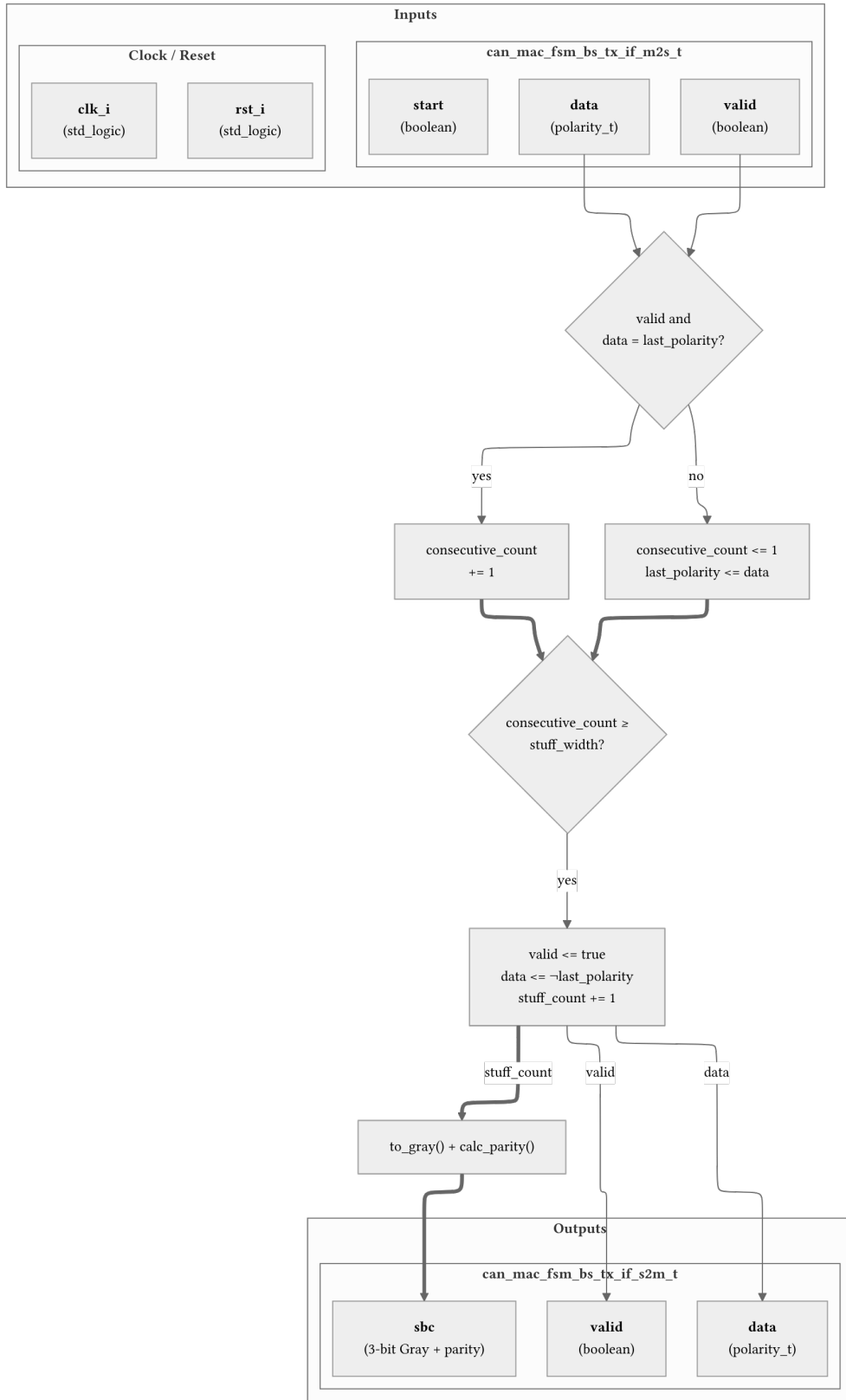
Figure 8: can_mac_bs_tx data path diagram. When valid and data = last_polarity , consecutive_count increments. Otherwise it restarts at 1 with last_polarity updated to data . When consecutive_count reaches stuff_width , valid and inverted data are driven and stuff_count increments. The to_gray() + calc_parity() block encodes stuff_count into the sbc output. All registers are clocked by clk_i . A rst_i or start pulse resets consecutive_count and stuff_count to zero. All outputs are registered.
