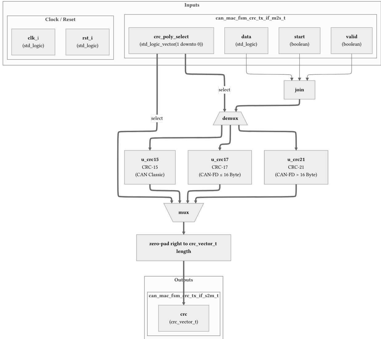
Figure 9: can_mac_crc_tx data path diagram. data , valid , and start are joined and demuxed by crc_poly_select to gate only the selected CRC engine. The mux selects the active engine result, which is zero-padded to the common erc_vector_t width. All registers are clocked by clk_i and cleared by rst_i . All outputs are registered.
