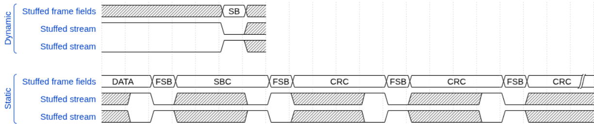
Figure 6: Dynamically and statically bit-stuffed data stream examples. In frame fields encoded with dynamic bit-stuffing an opposite polarity stuff bit (SB) is inserted after five consecutive same-polarity bits. In frame fields encoded with static bit-stuffing (SBC and CRC in FD frames) a fixed stuff bit (FSB) is inserted after each fourth bit. A FSB is also inserted before the first bit of the SBC field.
