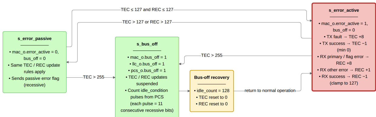
Figure 15: can_fce FSM (ISO 11898-1 sec. 8.1.4.4, Figure 43). s_error_active is the initial state after reset_i or llc_i.normal_mode. When TEC exceeds 127 or REC exceeds 127 the FCE moves to s_error_passive, clearing mac_o.error_active. If TEC exceeds 255 from either active or passive state, the FCE enters s_bus_off, asserting bus_off to the MAC, LLC, and PCS. Recovery counts 128 idle_condition pulses from the PCS (each pulse represents 11 consecutive recessive bits); on the 128th pulse TEC and REC are reset to zero and the FSM returns to s_error_active.
