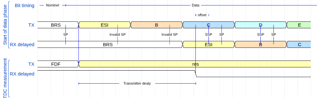
Figure 6: Transmitter Delay Compensation (TDC). At high data-phase bit rates the sum of bus propagation and transceiver delays ( t_{loop} ) may exceed one nominal bit time, causing the echo of a driven bit to arrive too late for the standard sample point. TDC measures this loop delay during the first data-phase bit and positions the Secondary Sample Point (SSP) at offset t_{SSP} = t_{TDC\_offset} + t_{measured} , so that each transmitted bit is verified against its bus echo at the correct moment. The SSP replaces the nominal SP for bit-error monitoring throughout the data phase [1, Sec. 7.3.4].
