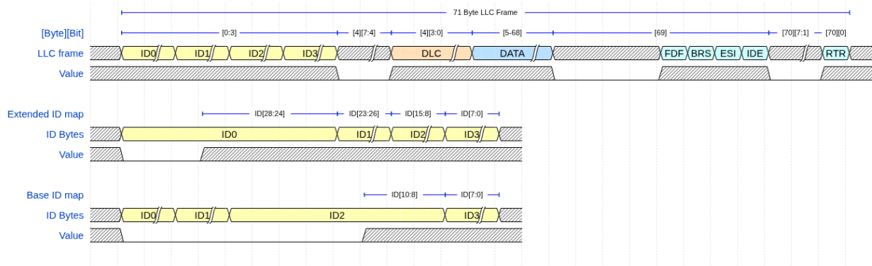
Figure 8: LLC frame format (71 bytes) at the host-MAC interface. Bytes 0-3 encode the identifier; byte 4 carries the frame-type selector FMT in bits [7:4] and DLC in bits [3:0]; bytes 5-68 carry up to 64 data bytes; byte 69 carries the FDF, BRS, ESI, and IDE control flags; byte 70 carries RTR in bit 0. The lower rows show the identifier byte mapping: for extended identifiers ID[28:24] are packed into ID0, ID[23:16] into ID1, ID[15:8] into ID2, and ID[7:0] into ID3; for base identifiers ID0 and ID1 are all zeros, ID[10:8] occupies the lower three bits of ID2, and ID[7:0] fills ID3.
