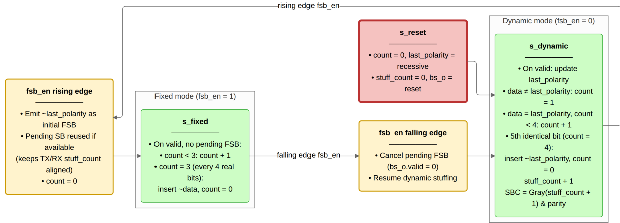
Figure 13: can_mac_bs (2 modes). Dynamic mode counts consecutive identical bits and emits an inverse stuff bit on the 5th (count = 4), updating the Gray-coded SBC. Fixed mode is entered on the rising edge of fsb_en, which immediately emits the initial FSB; thereafter one FSB is emitted every 4 real bits (count = 3). The falling edge of fsb_en cancels any pending FSB and returns to dynamic mode. stuff_count and the SBC output are maintained continuously across both modes.
