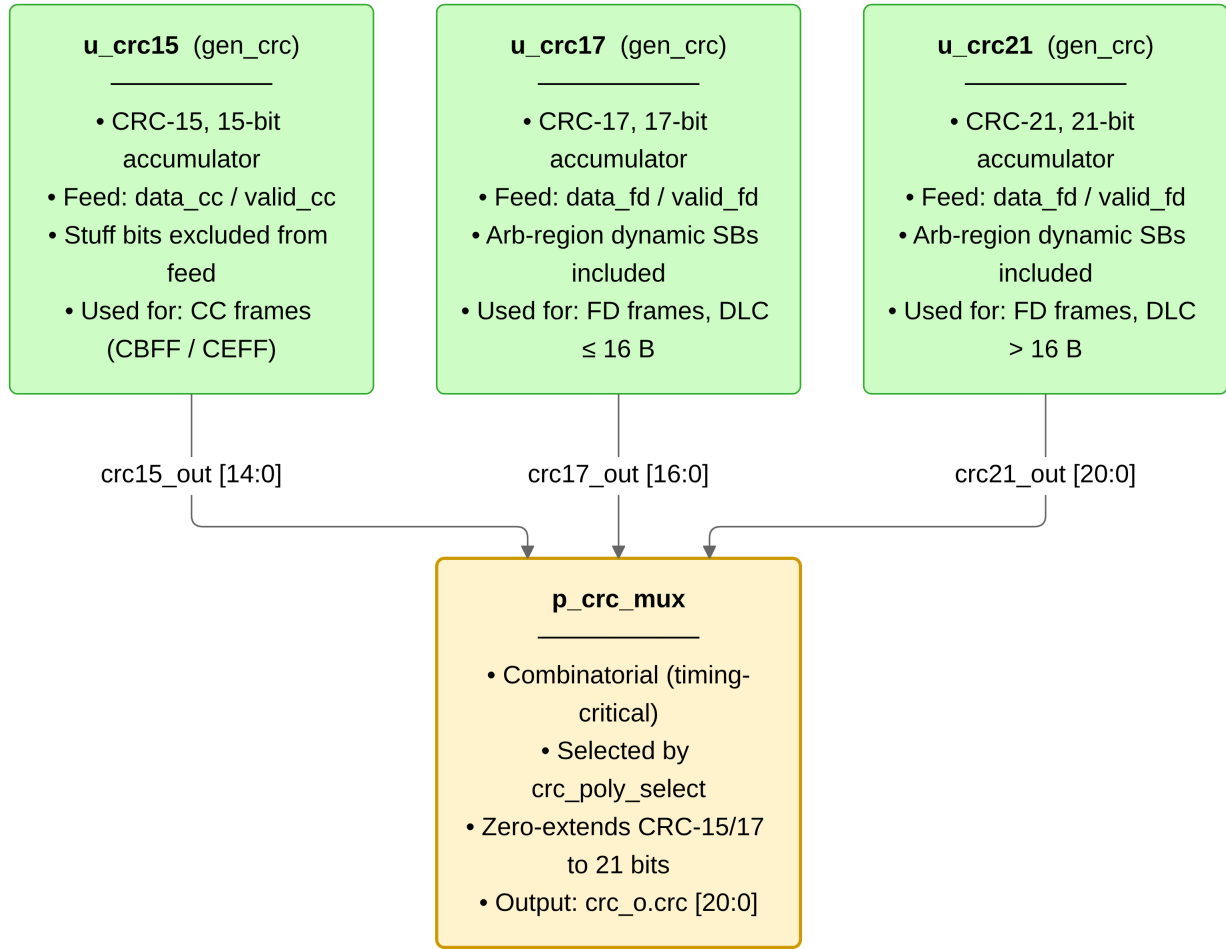
Figure 14: can_mac_crc dataflow. Three gen_crc instances accumulate in parallel on every clock: u_crc15 is fed by data_cc/valid_cc (CC bit stream, stuff bits excluded); u_crc17 and u_crc21 are both fed by data_fd/valid_fd (FD bit stream, dynamic stuff bits included in the arbitration region). The combinatorial mux p_crc_mux selects the active engine result based on crc_poly_select and zero-extends it to the common 21-bit output. reset_i reinitializes all three engines simultaneously.
