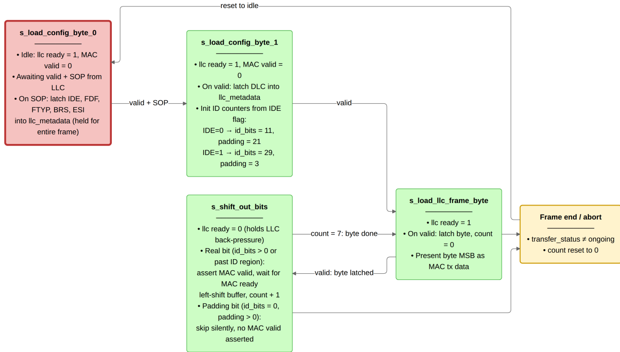
Figure 12: can_mac_ser (4 states). Config bytes carry frame metadata (IDE, FDF, FTYP, BRS, ESI, DLC); these are latched once and held stable for the entire frame. In s_shift_out_bits real ID and data bits are driven one per MAC FSM ready pulse, while unused padding bits in the 32-bit ID field are skipped silently. Any transfer_status \neq ongoing signal from the MAC FSM returns the serializer to s_load_config_byte_0 from any state.
