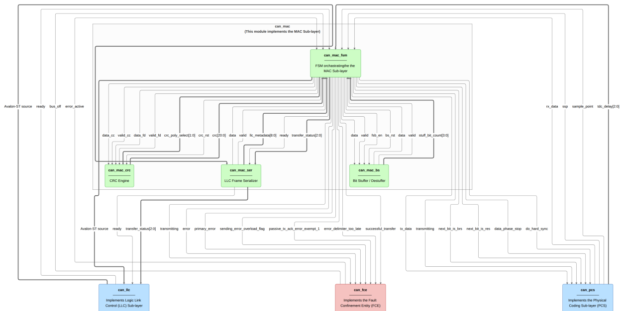
Figure 10: ‘can_mac’ architecture. Individual signals are shown on each directed edge, matching the signal names used in the sub-module diagrams. MAC-internal connections: ‘can_mac_ser_tx’ feeds the serial bit stream and ‘llc_metadata’ to ‘can_mac_fsm’; ‘can_mac_bs’ accepts ‘data/valid/fsb_en’ and returns stuffed ‘data/valid’ plus the Gray-coded ‘stuff_bit_count’ for the SBC field; ‘can_mac_crc’ receives the dual CC/FD bit feeds and returns the running ‘crc[20:0]’ digest. External connections: ‘can_llc’ connects to the MAC on both TX (‘tx_llc_i/o’ via the serializer) and RX (‘rx_llc_i/o’ via the FSM); bit-level timing to ‘can_pcs’ (‘tx_data’, ‘rx_data’, sample-point strobes); fault-confinement events to/from ‘can_fce’ (‘error_active’, ‘bus_off’). Full interface definitions: can_mac_ser_fsm_if (Table ??), can_mac_fsm_bs_if (Table ??), can_mac_fsm_crc_if (Table ??).
