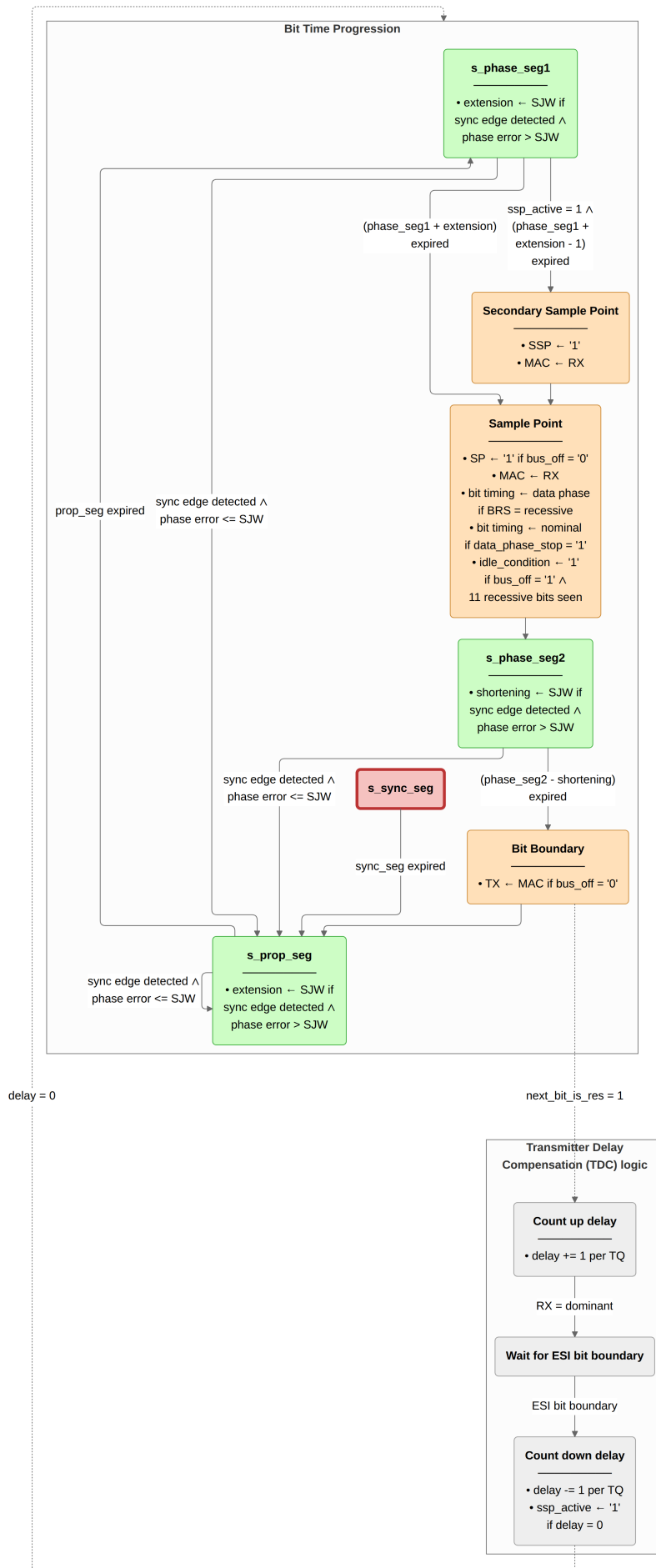
Figure 16: can_pcs operation (ISO 11898-1 sec. 7.2-7.4). Two concurrent-per-TQ blocks are shown alongside the main bit time progression. The bit time progression (green, centre) cycles through s_sync_seg (1 TQ fixed), s_prop_seg, s_phase_seg1, and s_phase_seg2. A sync edge detected mid-segment triggers soft synchronization: with phase error at most SJW the bit time restarts from s_prop_seg; with larger
