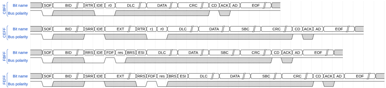
Figure 4: Classic CAN base frame (CB) and CAN FD base frame (FB) bit-field layouts. The FD frame extends the control field with FDF, res, BRS, and ESI between the IDE bit and the DLC; the data and CRC fields are transmitted at the data-phase bit rate when BRS is recessive.
