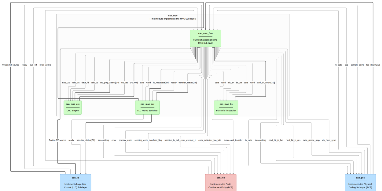
Figure 10: ‘ can_mac ’ architecture. Individual signals are shown on each directed edge. MAC-internal connections: ‘ can_mac_ser_tx ’ feeds the serial bit stream and ‘ llc_metadata ’ to ‘ can_mac_fsm ’; ‘ can_mac_bs ’ accepts ‘ data/valid/fsb_en ’ and returns stuffed ‘ data/valid ’ plus the Gray-coded ‘ stuff_bit_count ’ for the SBC field; ‘ can_mac_crc ’ receives the dual CC/FD bit feeds and returns the running ‘ crc[20:0] ’ digest. External connections: ‘ can_llc ’ connects to the MAC on both TX (‘ tx_llc_i/o ’ via the serializer) and RX (‘ rx_llc_i/o ’ via the FSM); bit-level timing to ‘ can_pcs ’ (‘ tx_data ’, ‘ rx_data ’, sample-point strobes); fault-confinement events to/from ‘ can_fce ’ (‘ error_active ’, ‘ bus_off ’).
